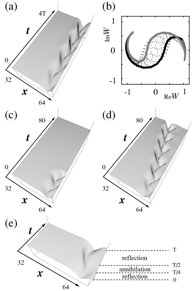
FIG. 5. (a) Spatiotemporal pattern of the scattor with the period T \approx 12.8730 at c_3 \approx 0.142\ 429 . (b) Phase portraits of the scattor: The solid (respectively gray) line indicates the interface when t = 3T/8 (respectively t = 5T/8 ). (c) [respectively (d)] Response of the scattor by adding a small constant-multiple perturbation of \Phi to the snapshot of the unstable orbit at t = 3T/8 (respectively t = 5T/8 ). (e) Phase-dependent response of the scattor.
