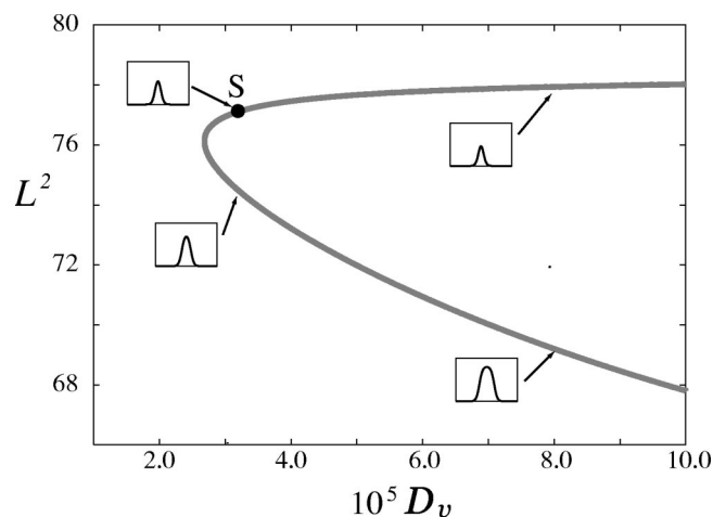
FIG. 12. Continuation of the scattor S corresponding to Fig. 11(A) with D_v being a bifurcation parameter and r_c = 9.6 \times 10^{-4} . The branch turns back at a saddle-node (SN) point D_v = 2.68254 \times 10^{-5} .
