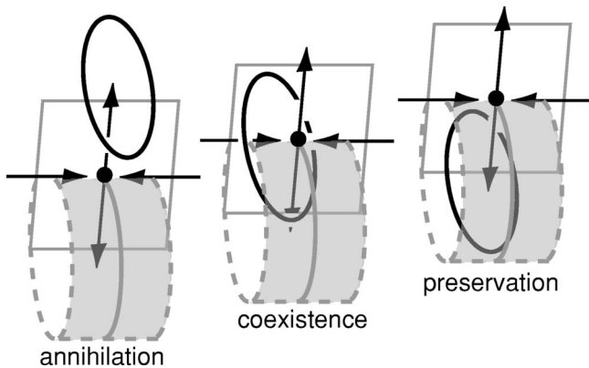
FIG. 7. Schematic picture of the relation for the plot of the profiles of the orbits right after collisions and the stable manifold of the time-periodic scattor of codim 1. The rectangle shows a Poincaré section of the scattor. The solid circle indicates the plot of profiles of the orbit as the collision-phase varies from 0 to 2\pi . It crosses the stable manifold of the scattor transversally as c_3 passes the transition point. Generically there is a nonempty interval of c_3 in which the circle belongs to both sides of the stable manifold of the scattor, which explains the outputs of Fig. 1(B)(c).
