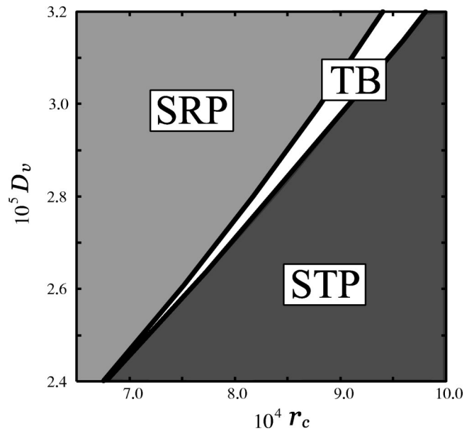
FIG. 8. Phase diagram in (r_c \times 10^4, D_v \times 10^5) space starting from a single pulse. SRP: self-replicating pattern. STP: stable traveling pulse. For parameters in SRP, each pulse undergoes backfiring.
