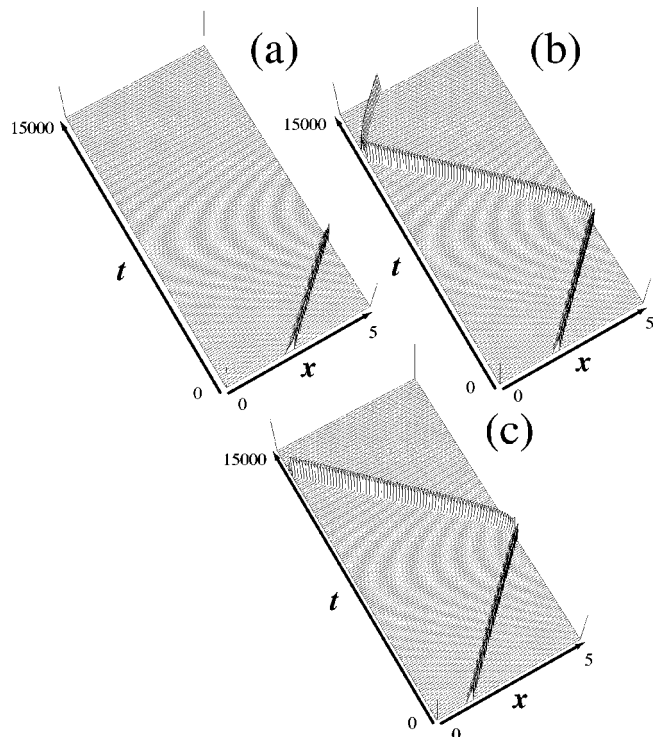
FIG. 9. Symmetric head-on collisions for the three-component system (3) (i.e., hitting the boundary with the Neumann condition). (a) Annihilation D_v=2.6 \times 10^{-5} , r_c=7.52 \times 10^{-4} . (b) Preservation D_v=3.2 \times 10^{-5} , r_c=9.72 \times 10^{-4} . (c) The output changes depending on the phase at collision: the first one is of preservation and the second one is of annihilation. D_v=3.19 \times 10^{-5} , r_c=9.60 \times 10^{-4} Only u component is displayed here.
