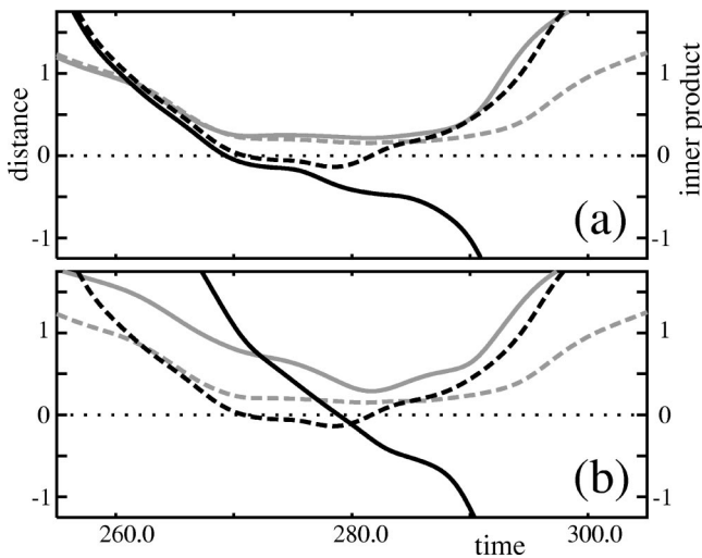
FIG. 6. Time evolutions of the inner product and distance to the scattor. (a) The inner product changes the sign from positive to negative when c_3 is decreased (solid black for c_3=0.14242 and solid gray for c_3=0.14244 ). The associated broken curves represent the distance to the scattor. (b) For an appropriate c_3 , the response depends on the phase of the initial breather as in Fig. 7. The inner product and associated distance are shown for two typical initial conditions (black and gray) with c_3=0.14244 . Solid (respectively broken) curves indicate inner product (respectively distance to the scattor).
