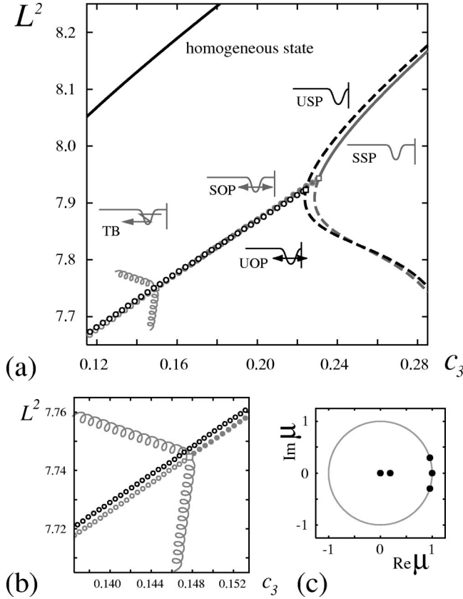
FIG. 4. (a) Global bifurcational origin of the time-periodic scattor. The bifurcation parameter is c_3 . The black open (respectively gray filled) circles indicate the unstable oscillating pulse (UOP) [respectively stable (SOP)] connected to USP (respectively SSP). TB emerges below c_3 \approx 0.148 . The solid line at the top of the figure indicates the stable uniform state. (b) A detail near the NS bifurcation point. (c) The distribution of multipliers \mu of SOP at c_3 \approx 0.148\ 022 . The gray circle shows |\mu|=1 .
