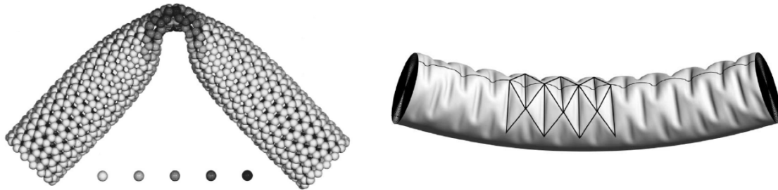
Figure 1: (Left) Kink structure formed in a single-walled nanotube under bending (Iijima 1996). (Right) Morphology of a rippled multi-walled nanotube reminiscent of the Yoshimura pattern. The ridges and furrows are highlighted, as well as the trace of the longitudinal section (Arroyo 2003).
