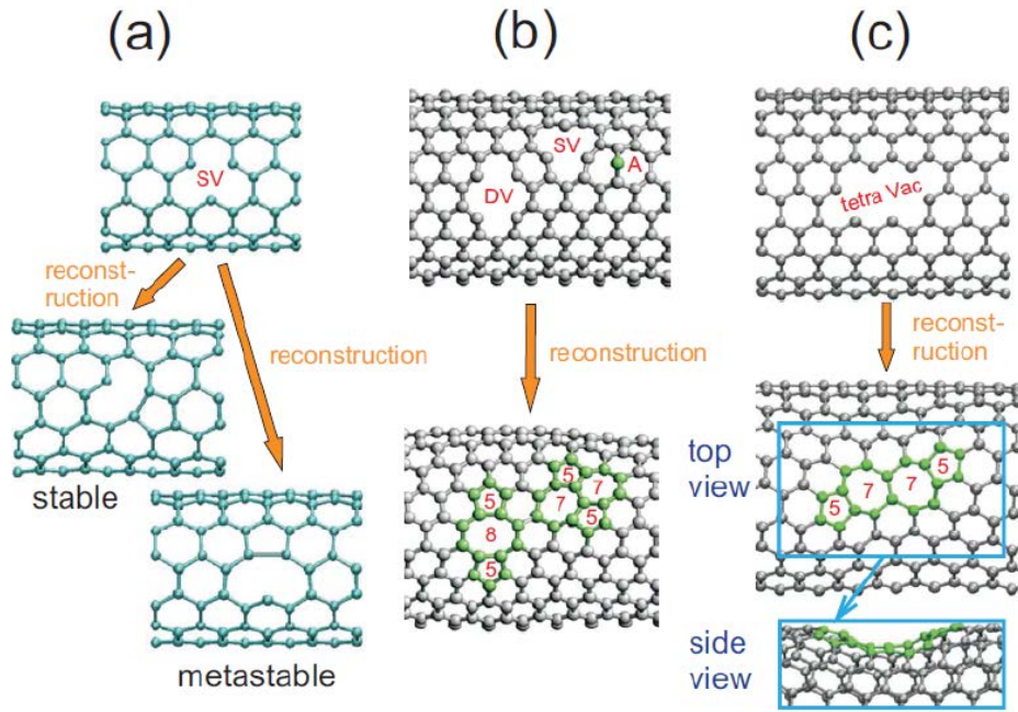
Figure 2: Reconstruction of the atomic network near vacancies produced by electron-beam irradiation. (a) A single vacancy (SV) state tends toward stable or metastable configurations depending on the orientation of the new weak pentagon bond. (b) A divacancy (DV) transforms to an agglomeration of five- and eight-membered rings. A SV and an adatom may form a metastable 5-7-7-5 defect. (c) Reconstruction of a tetravacancy. The effective size of the “hole” decreases at the expense of local diameter reduction (Krasheninnikov 2010).
