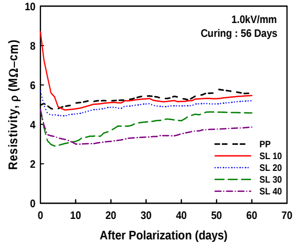
Figure 5: Age effect for \rho at 56 curing days.
