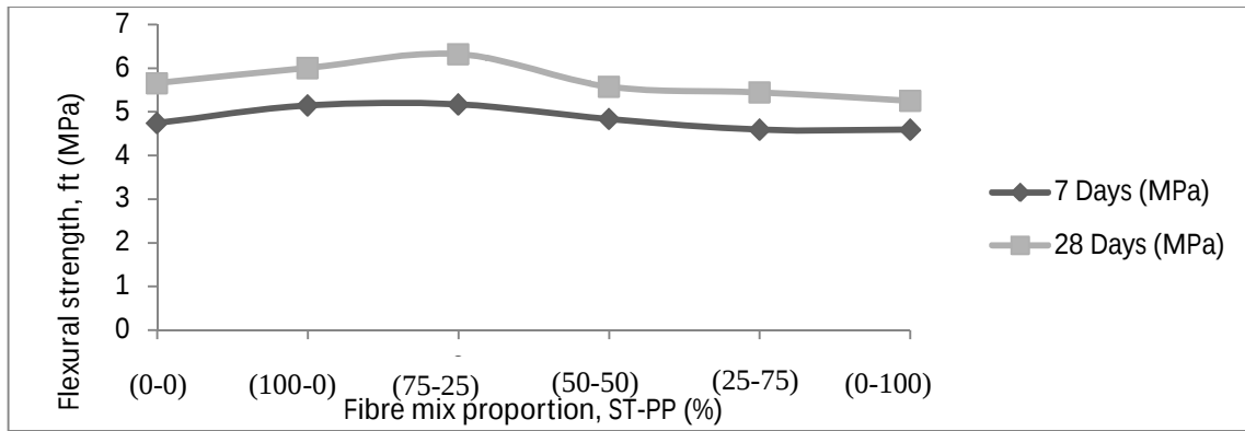
Figure 7: Flexural strength
