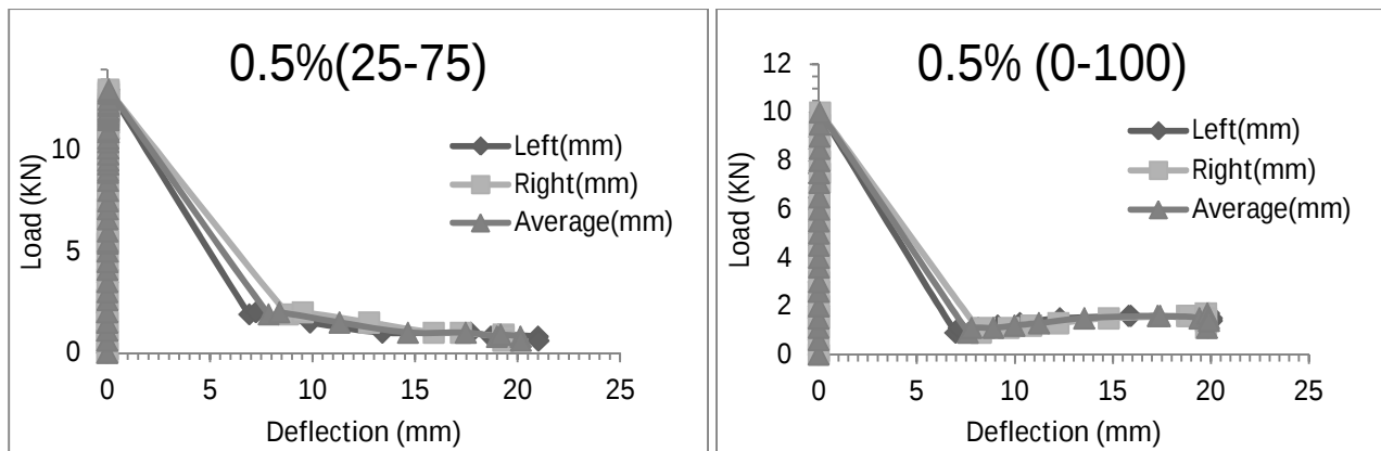
Figure 9: Load against deflection graph for every batch (Cont.)
