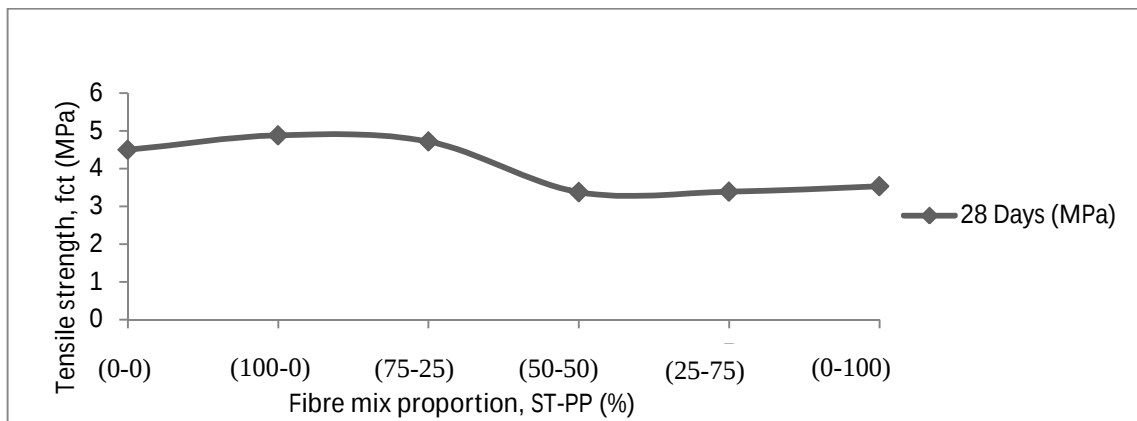
Figure 8: Tensile strength
