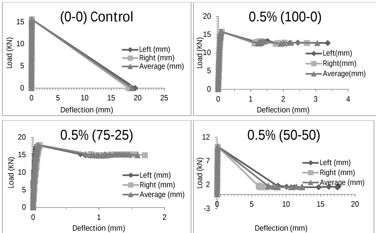
Figure 9: Load against deflection graph for every batch
