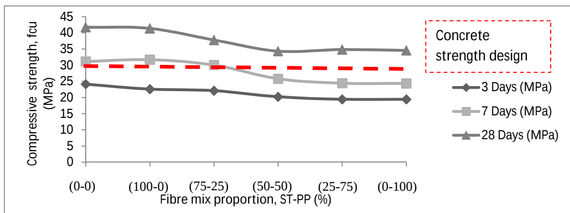
Figure 6: Compressive strength
