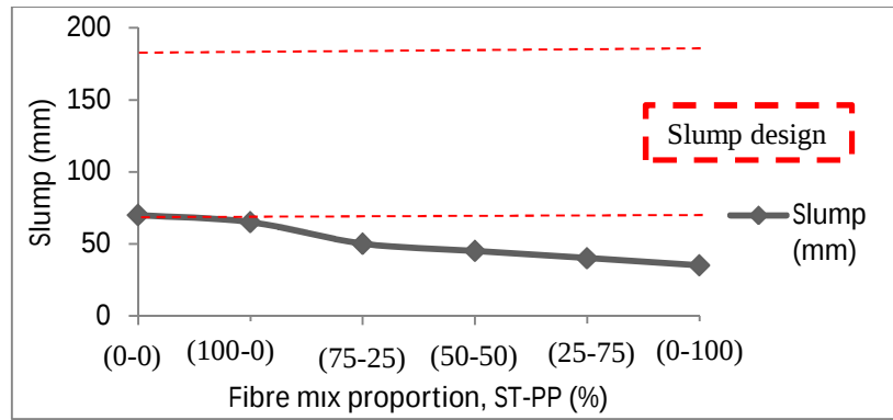
Figure 4: Slump result
