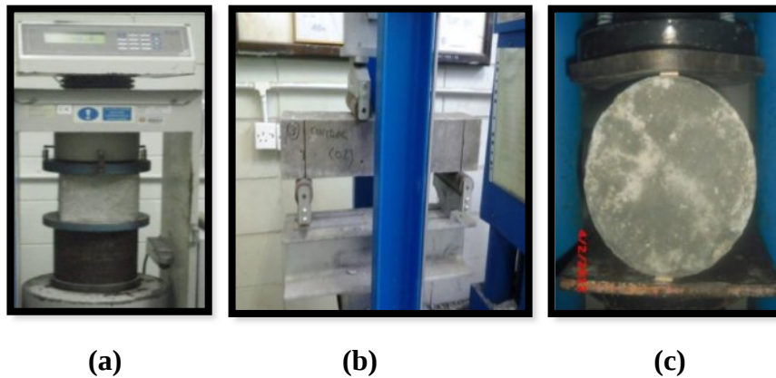
Figure 2: Test setup for the mechanical properties of HyFRCC: (a) Compressive, (b) flexural tensile and (c) splitting tensile
