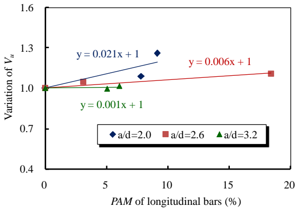
Figure 4: V_c - PAM relationships
