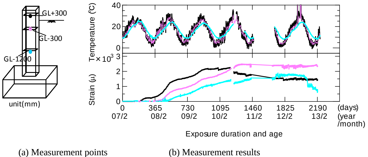
Fig. 3 Time variation of steel strain and temperature in column
