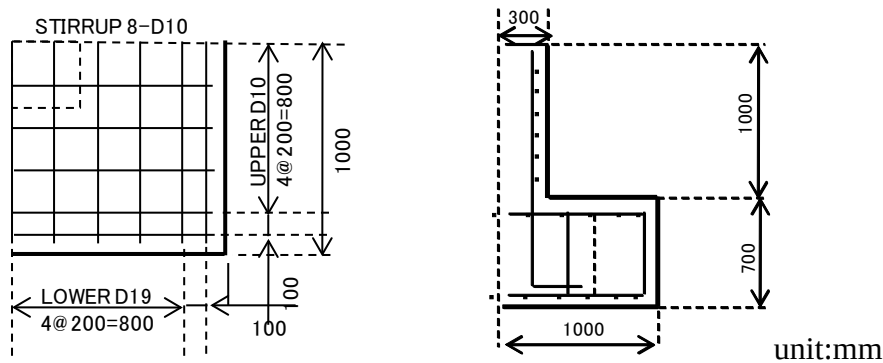
Fig. 1 Drawing showing dimensions and bar arrangement of footing models (For Cases 1 and 2. Left: plane section for footing, Right: vertical section)
