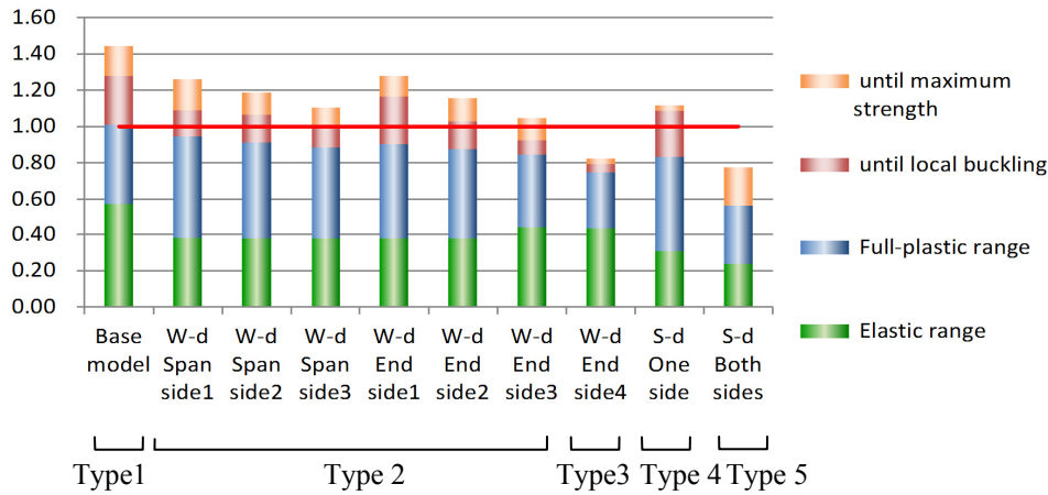
Figure 9: Summary of various limit strengths
