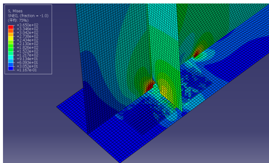
Figure 7: Examples of Initial yield strength Mises equivalent stress distribution
