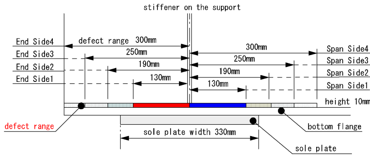
Figure 4: The used deficit parameters in the model
