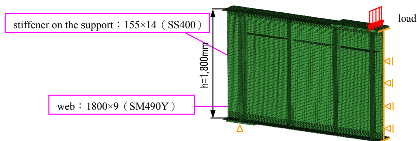
Figure 3: Overview of the model
