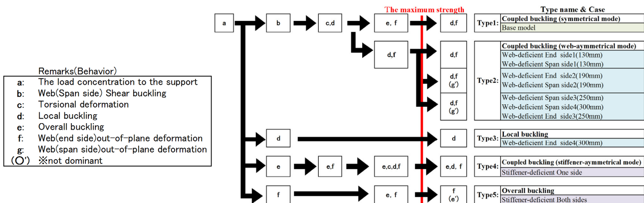
Figure 6: Classification of collapse mode
