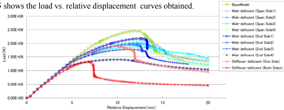
Figure 5: The load vs. relative displacement curves
