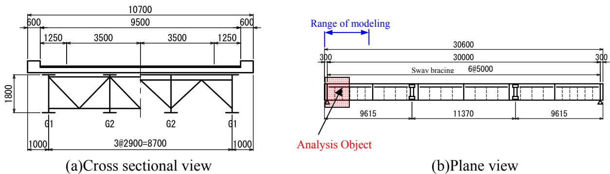
Figure 2: The objective girder end (unit :mm)
