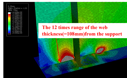
Figure 8: Examples of Full-plastic strength Mises equivalent stress distribution
