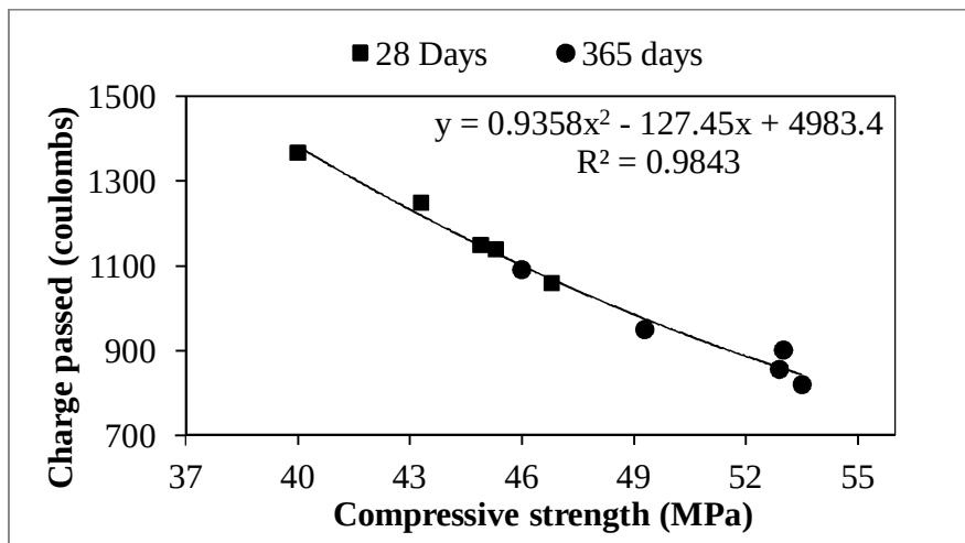
Figure 4: Compressive Strength verses RCPT
