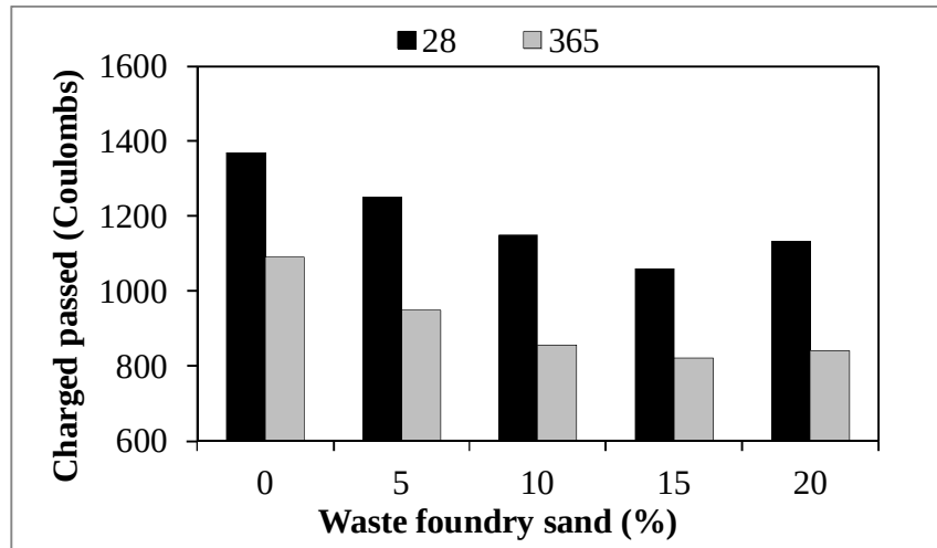
Figure 3: RCPT verses Waste Foundry Sand
