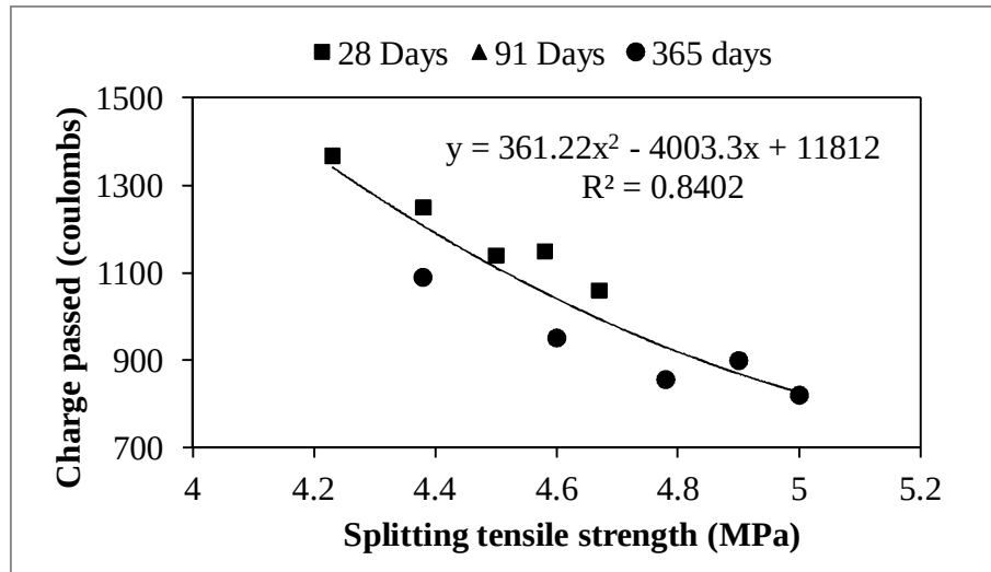
Figure 5: Splitting Tensile Strength verses RCPT
