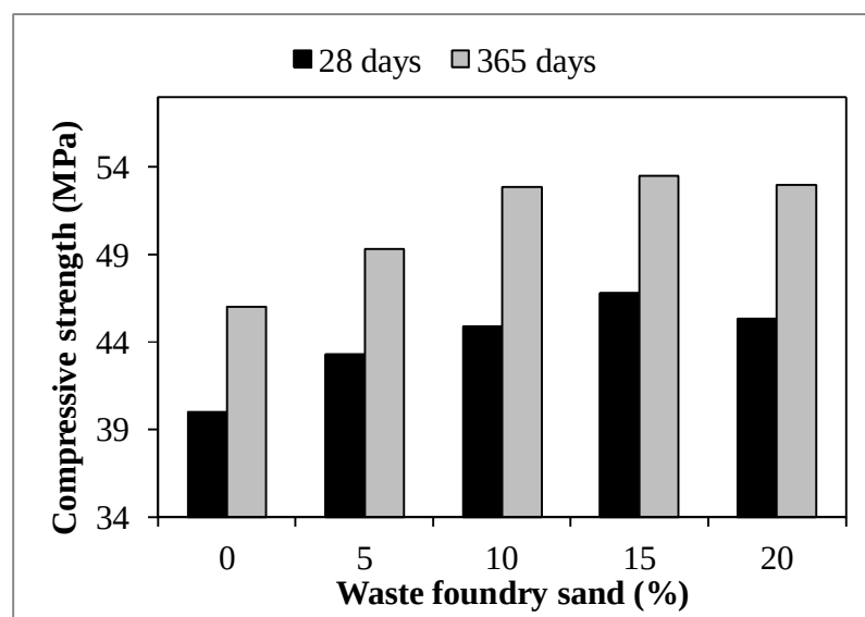
Figure 1: Compressive Strength verse Waste Foundry Sand
