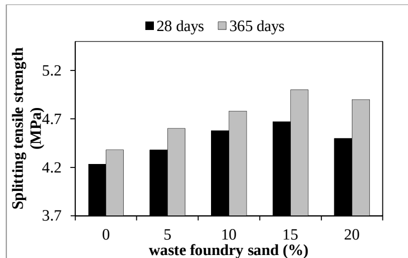
Figure 2: Splitting Tensile Strength verses Waste Foundry Sand
