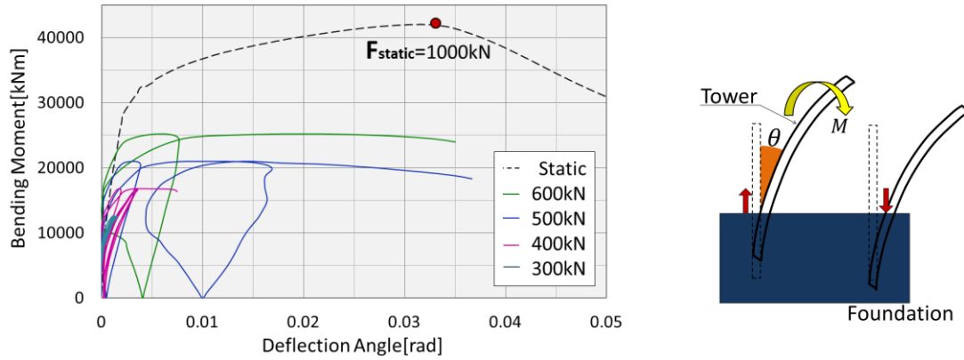
Figure 3: Relation of the bending moment to the deflection angle
