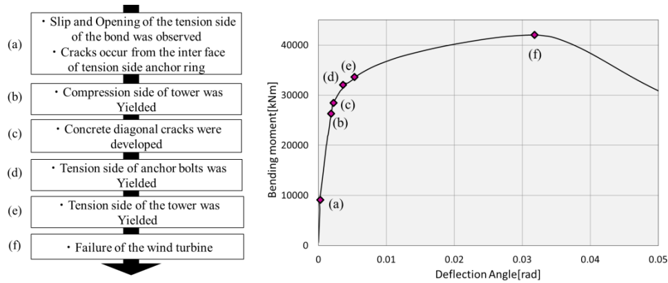
Figure 2: Failure process for static analysis
