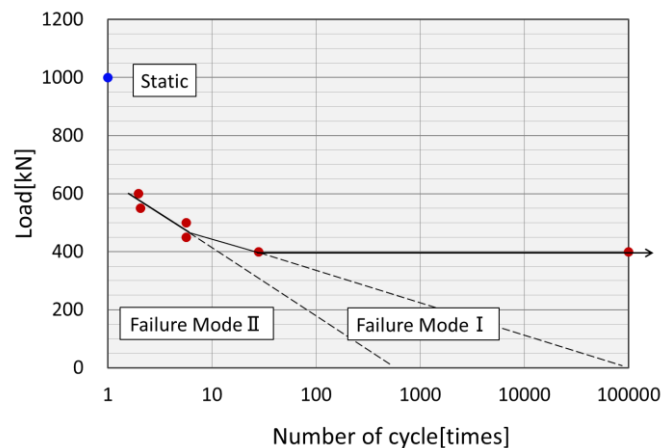
Figure 7: Load – Number of cycle
