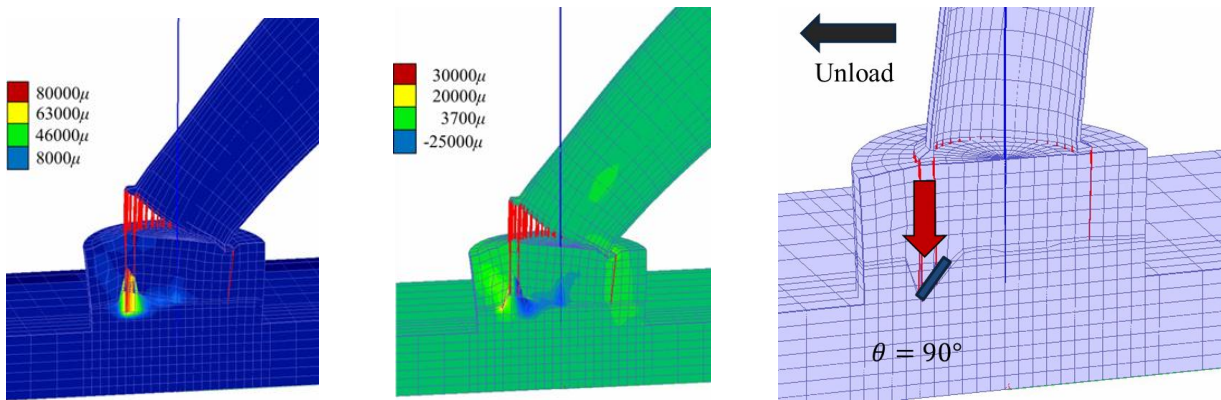
(a) Principal strain contour (b) Shear strain contour (c) Magnified deformation (disp. x50) (Just before failure)
