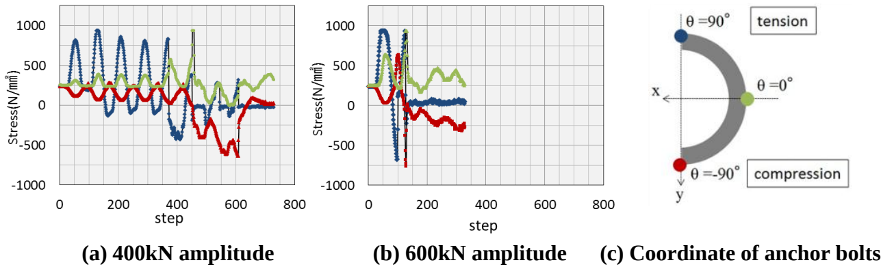
Figure 4: Stress of the anchor
