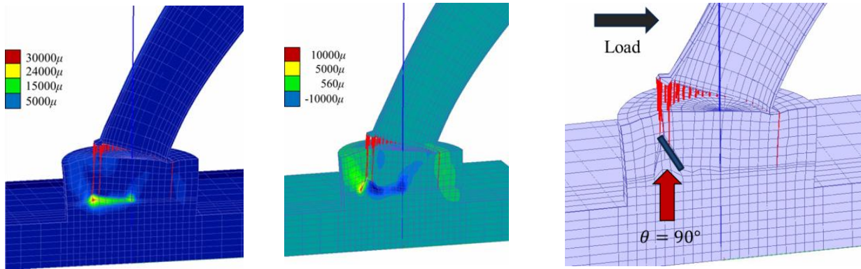
(a) Principal strain contour (b) Shear strain contour (c) Magnified deformation (disp. x50)
