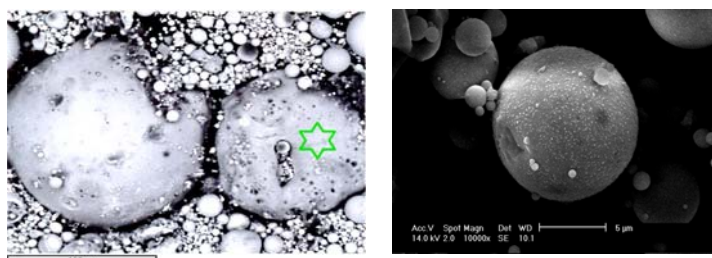
Particle shape of High calcium oxide fly ash(left) and low calcium oxide fly ash (right)
