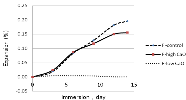
Fig.3 Expansion of mortar bar with different fly ash types
