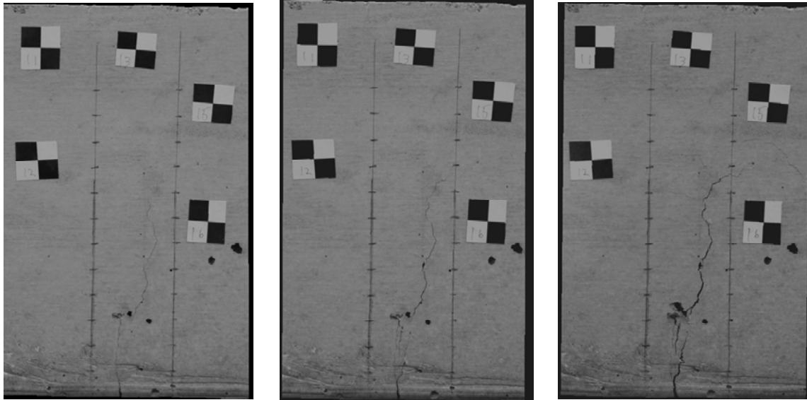
Figure 7: Ortho images (left image: projected result in STEP3, center image: projected result in STEP4, and right image: projected result in STEP5).
