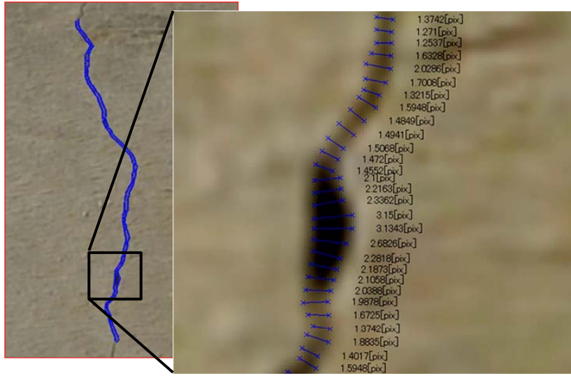
Figure 8: Automated crack extraction result.
