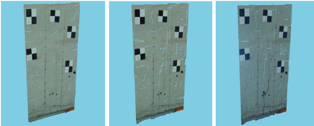
Figure 9: Point cloud generation results using close-range stereo (left image: point cloud after STEP3, center image: point cloud after STEP4, and right image: point cloud after STEP5).
