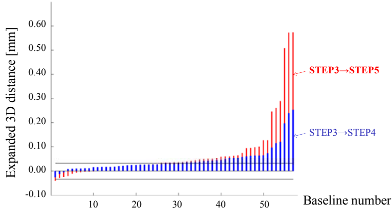
Figure 5: Relative 3D displacements on verification baselines.
