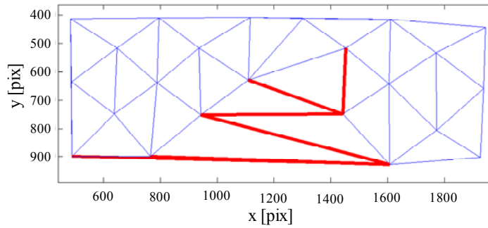
Figure 6: Verification baselines that show relative 3D displacements greater than 0.15 mm.
