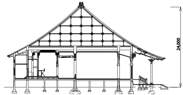
Figure 3: Section View (unit: mm)
