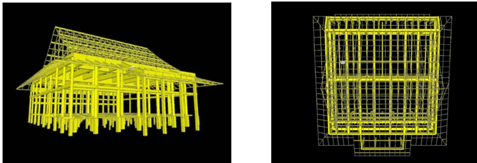
Figure 8: Analytical model of the temple
