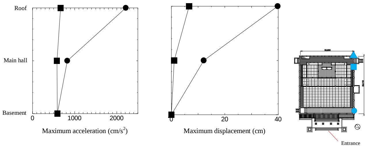
Figure 9: Seismic response analysis results
