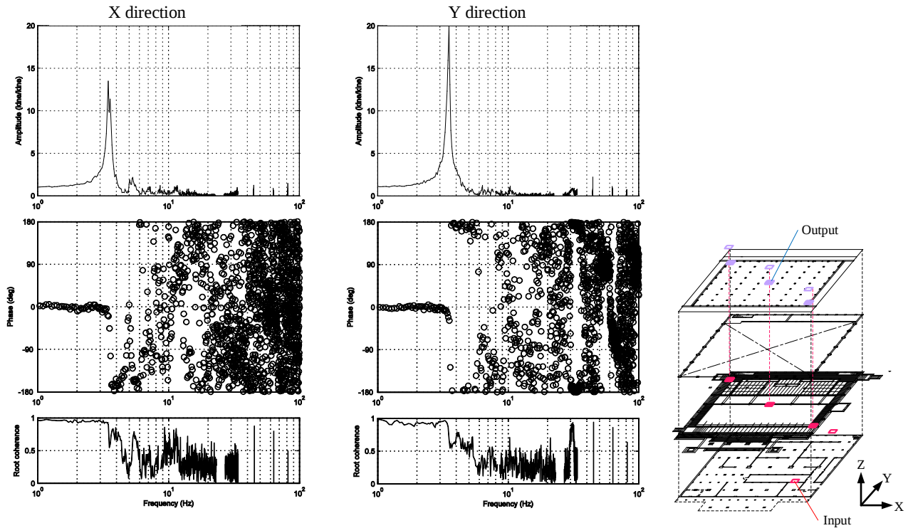
Figure 7: Transfer function (amplitude, phase and root coherence)
