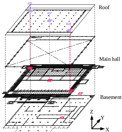
Figure 6: Sensor configuration
