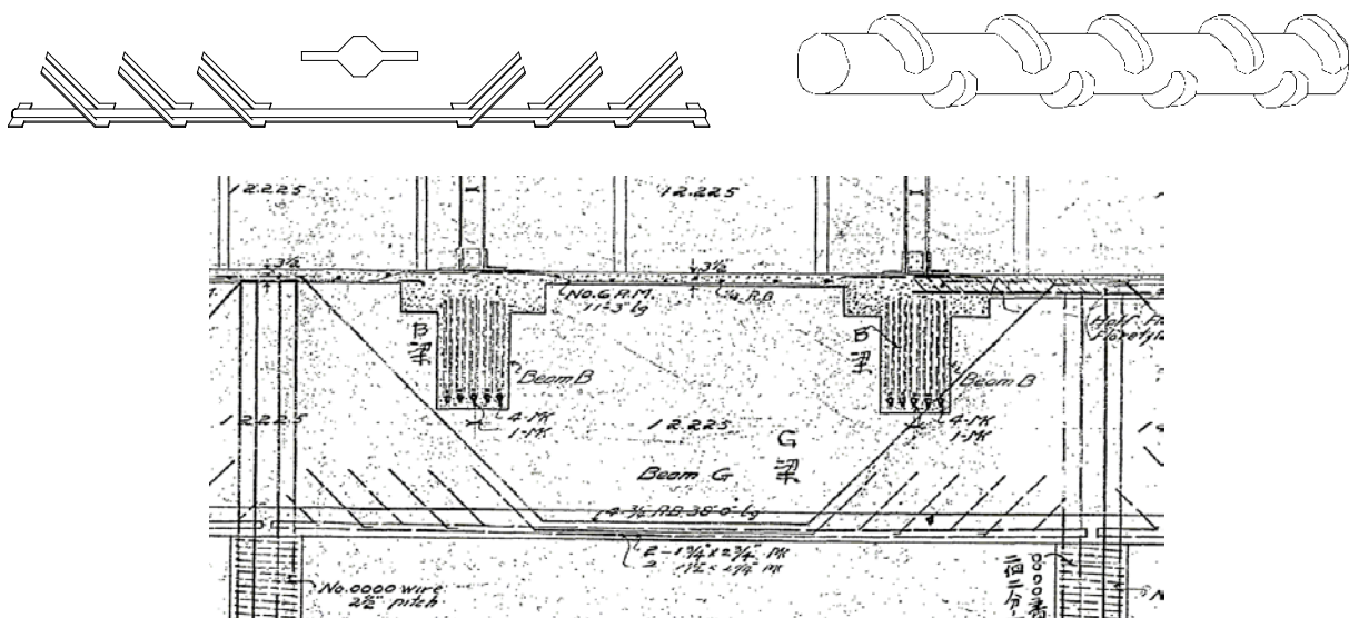
Figure 4: Kahn system
