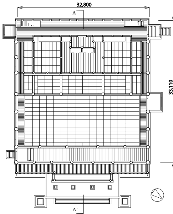
Figure 2: Plan view of the main floor (unit: mm)
