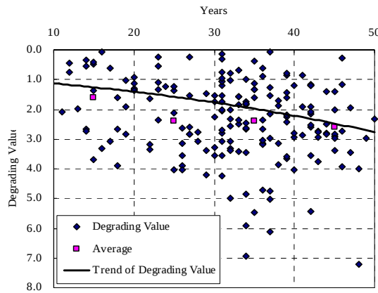
Figure3: Degrading and Average Value of Tunnel Lining.
