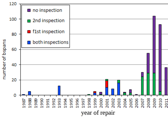
Fig. 2 Years and number of spans (379 in total) with partial slab repair since 1987
