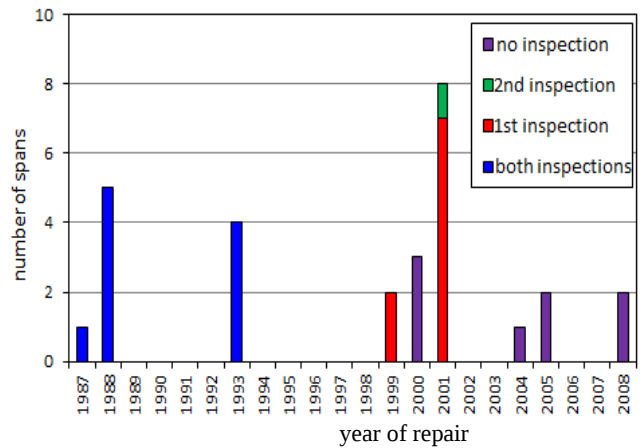
Fig. 3 Years and number of spans (28 in total) with full-length slab repair since 1987
