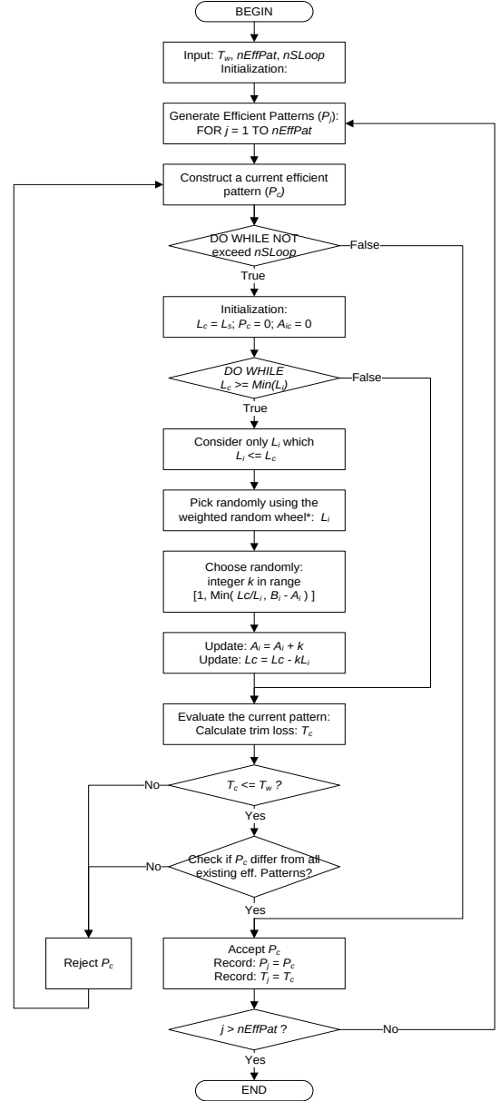
Figure 1: Pseudo-code and flowchart of Intensive Search Algorithm
