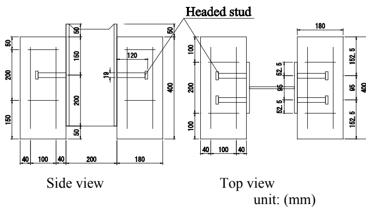
Figure 2: Specimen details
