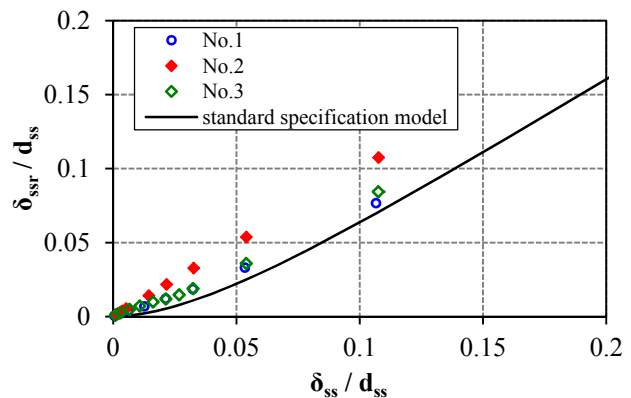
Figure 7: \delta_{ssr} - \delta_{ss} relationships of specimens
