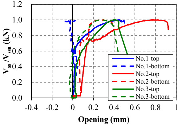
Figure 8: V_{ss}/V_{ssu} - opening relationships of specimens
