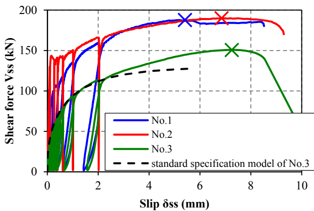
Figure 5: V- \delta relationships of specimens
