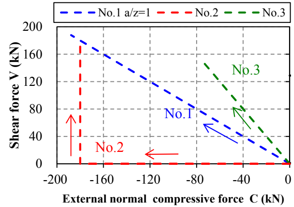
Figure 4: V-C relationship
