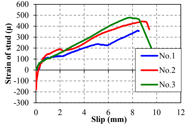
Figure 9: Strain -slip relationships of specimens
