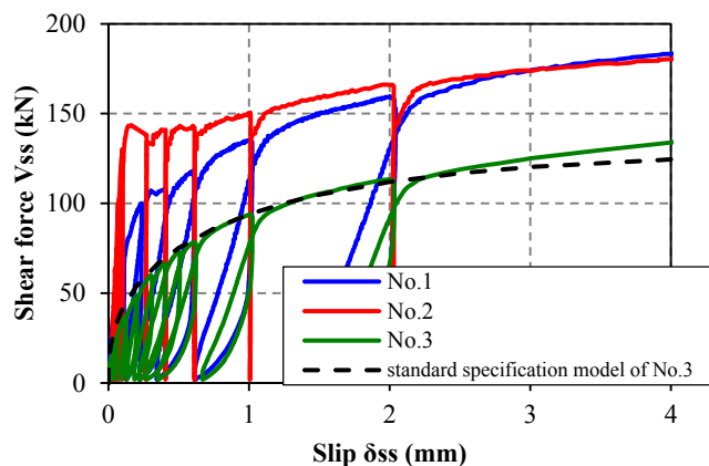
Figure 6: V- \delta relationships of specimens
