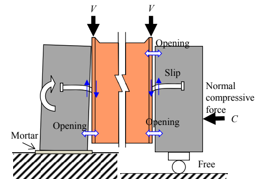
Figure 3: Specimen deformation during the test
