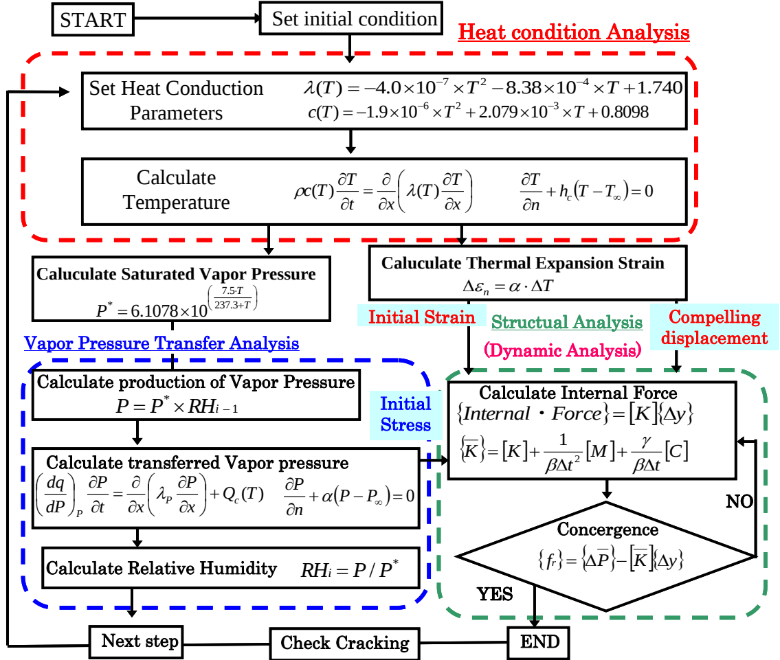
Figure 6: Analytical Flow
