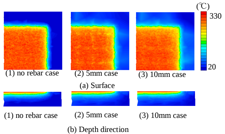
Figure 14: Temperature distribution
