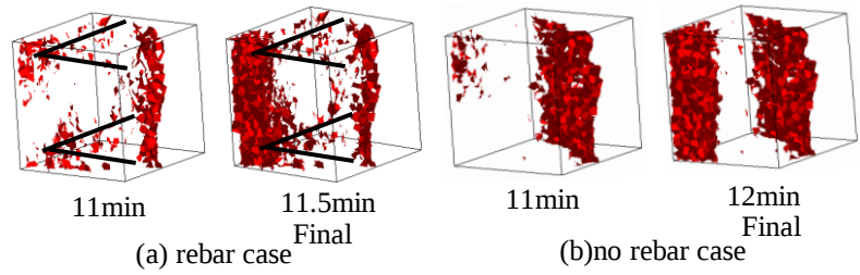
Figure 8 : Cracking behavior
