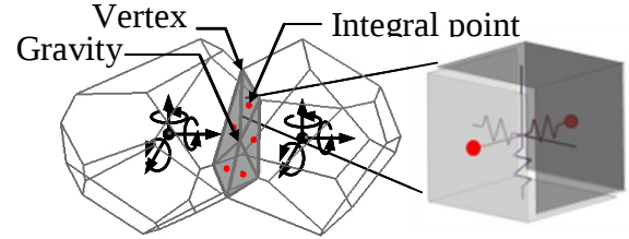
Figure 1 : Rigid Body Spring Model
