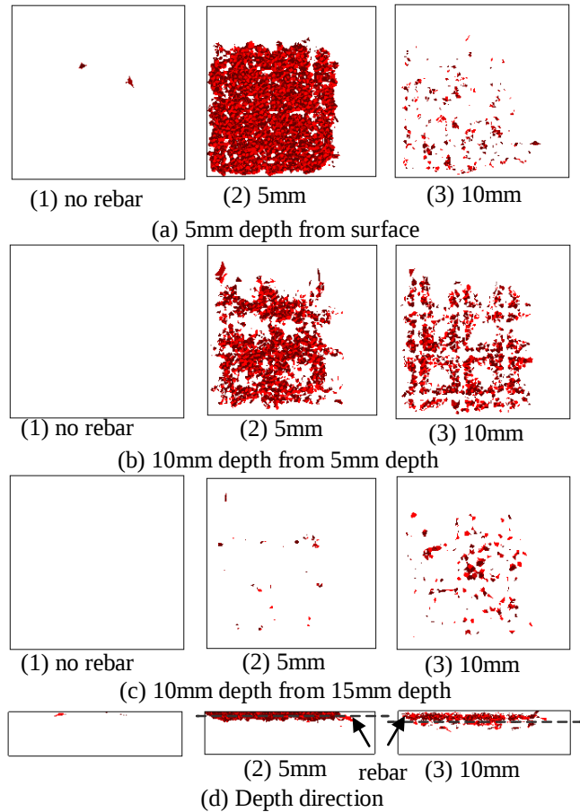
Figure 15: Cracking behavior
