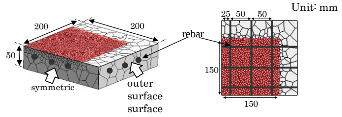
Figure 12: Analytical model
