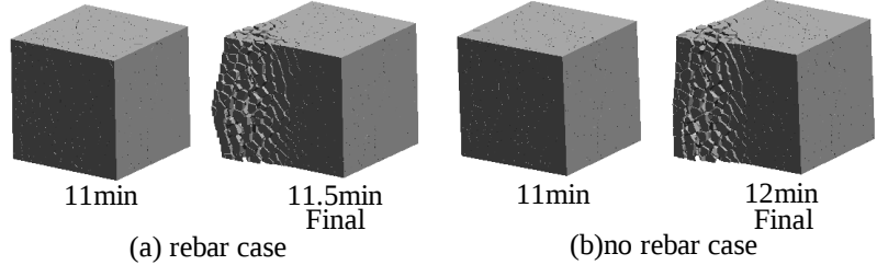
Figure 9 : Deformation behavior
