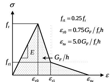
Figure 3: Stress-strain relationship
