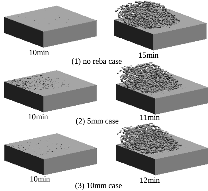
Figure 13 : Deformation behavior
