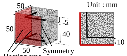
Figure 7: Analytical Model
