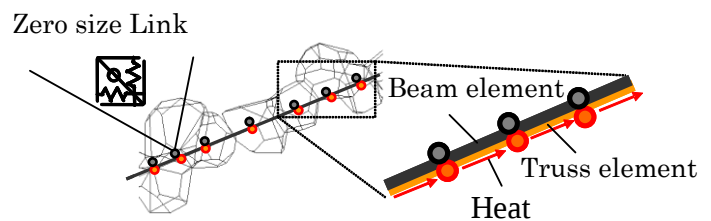
Figure 4: Modeling of rebar
