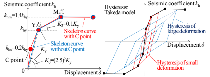
Figure 6: Non-linear spring characteristics
