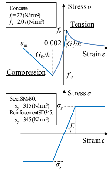
Figure 4: Relationship of stress-strain
