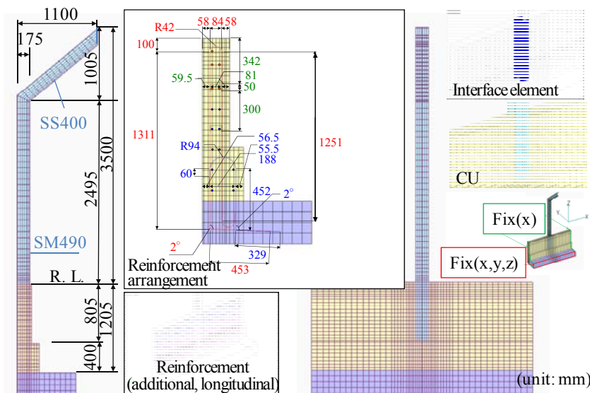
Figure 3: Analysis model of the detailed model (limit value)
