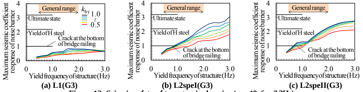
Figure 12: Seismic safety of target noise barrier ( \alpha_{nbr}=10, f_{nbr}=3.3\text{Hz} )
