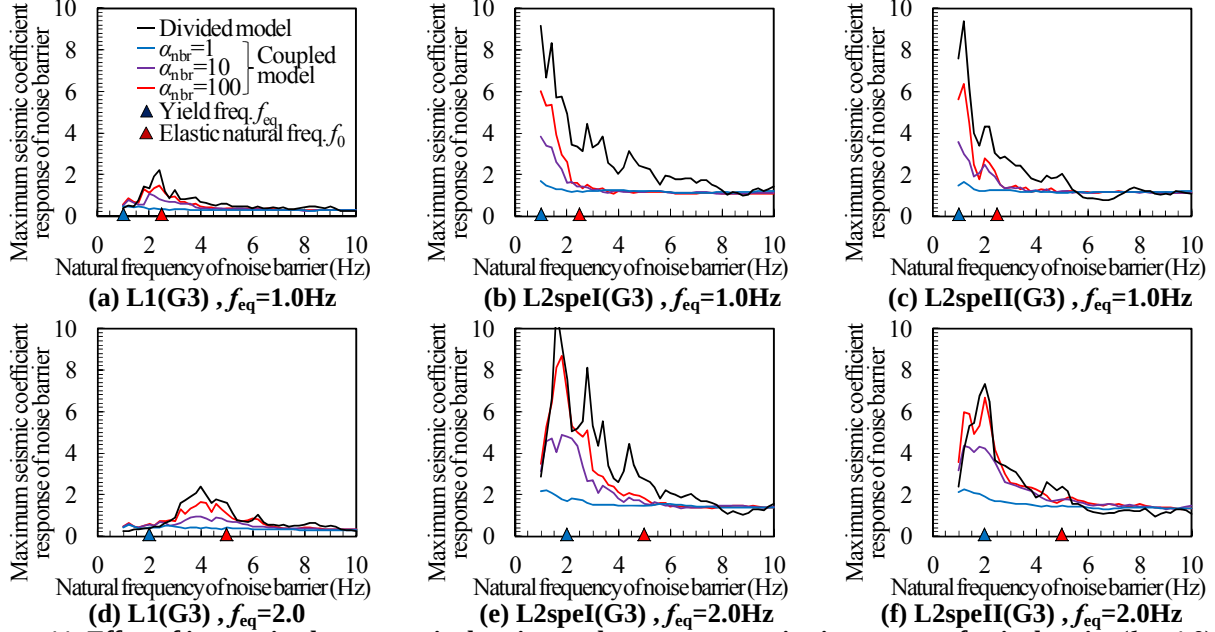
Figure 11: Effect of interaction between noise barriers and structures on seismic response of noise barrier ( k_{hy}=1.0 )
