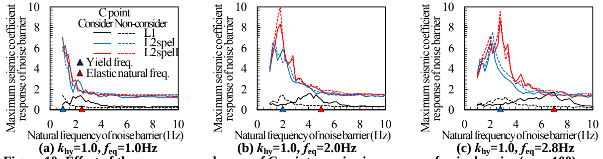
Figure 10: Effect of the presence or absence of C point on seismic response of noise barrier ( \alpha_{nbr}=100 )
