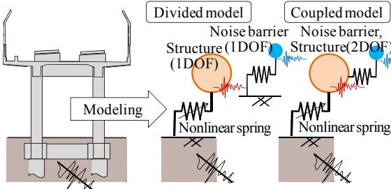
Figure 5: Analysis model of the detailed model (response value)
