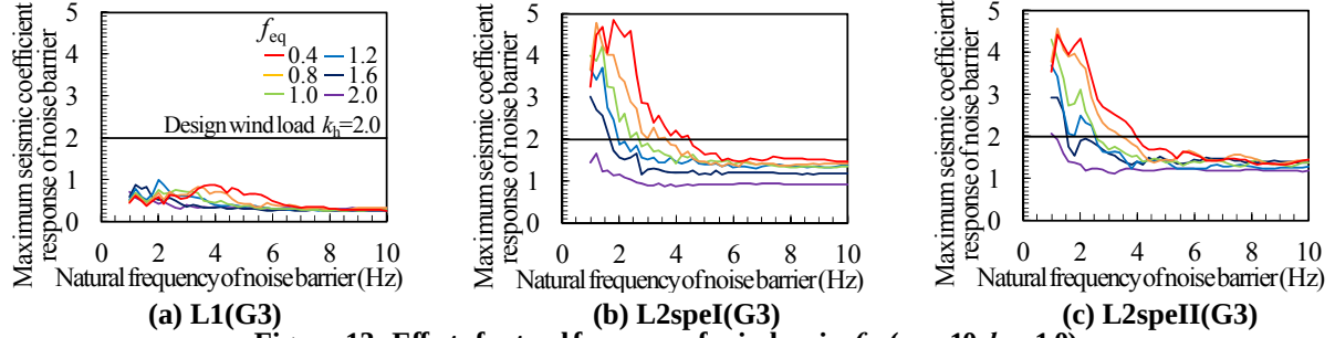
Figure 13: Effect of natural frequency of noise barrier f_{nbr} ( \alpha_{nbr}=10, k_{hy}=1.0 )
