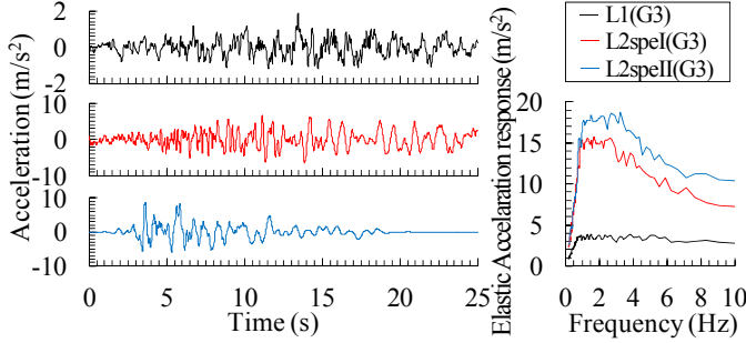
Figure 7: Time history waveforms and elastic response spectra of earthquakes
