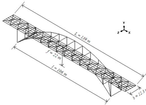
Figure 1: Theoretical arch model
