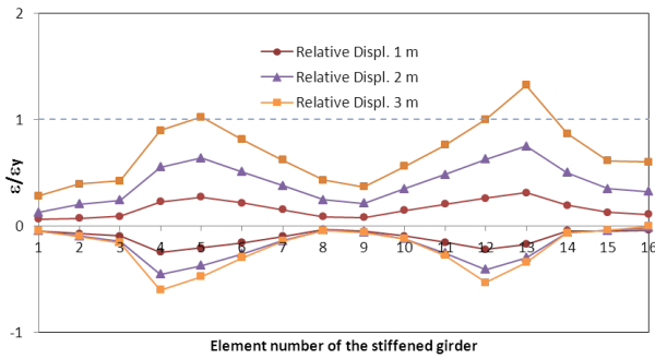
b) Stiffened girder
