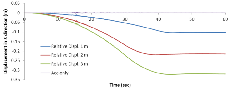
Figure 6: Displacement-time history response in X-direction (in acceleration direction) in Case I-a
