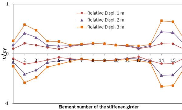
a) Stiffened girder
