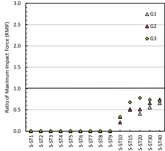
Figure 6: Pounding damage.
