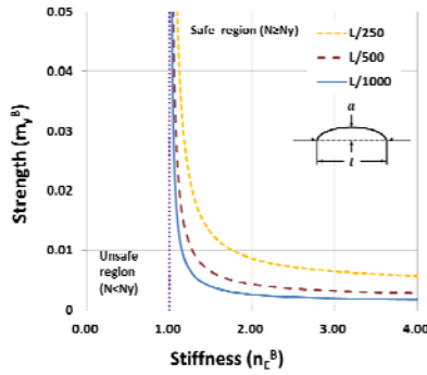
Figure 3 : Strength-Stiffness Graph
