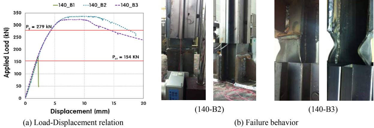
Figure 6: Load-Displacement relation and Failure behavior (140 Member)
