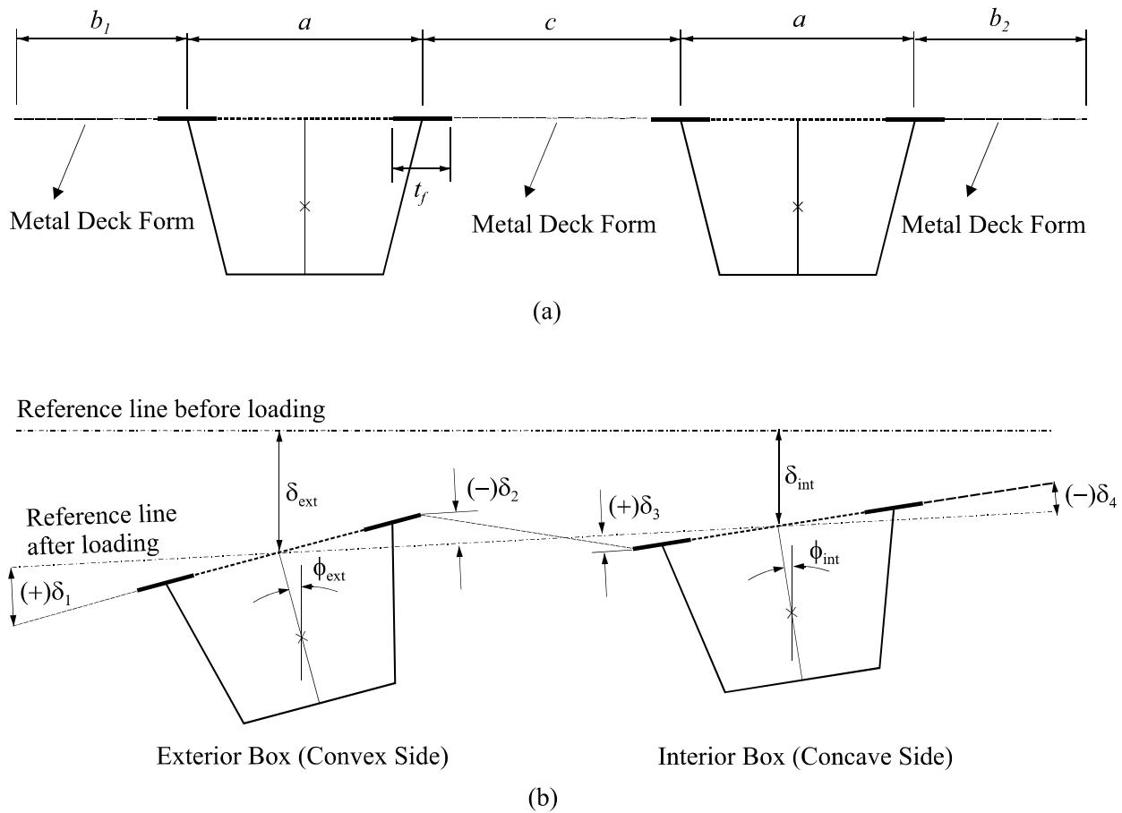
Figure 1: Twin-box-girder bridge cross-section: (a) Deck width; (b) Deformed shape.
