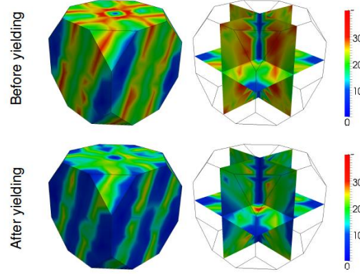
Figure 4: Coaxiality between crystal stresses and the closest SCYS vertex, \theta_c^v (Unit: deg.)
