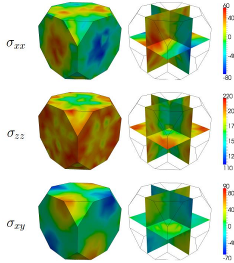
Figure 3: Crystal stress distribution over crystal orientation space after yielding ( \sum_{zz} = 180\text{MPa} , Unit: MPa)
