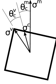
Figure 2: The schematic of crystal yield surface (SCYS). \sigma^c is the crystal stress, \sigma^v is the stress for a SCYS vertex, and \sigma^m is the macro-scale applied loading direction. The coaxiality between \sigma^c and \sigma^v or \sigma^m is defined by the angle \theta_c^v and \theta_c^m .
