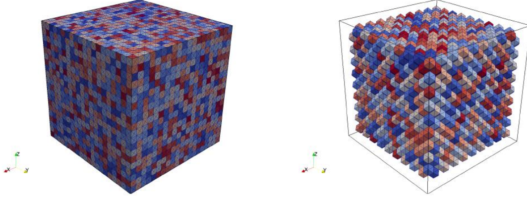
Figure 1: Finite element mesh. Total mesh (RVE) (left) and visualization of full dodecahedral grains by removing partial grains of RVE mesh (right).
