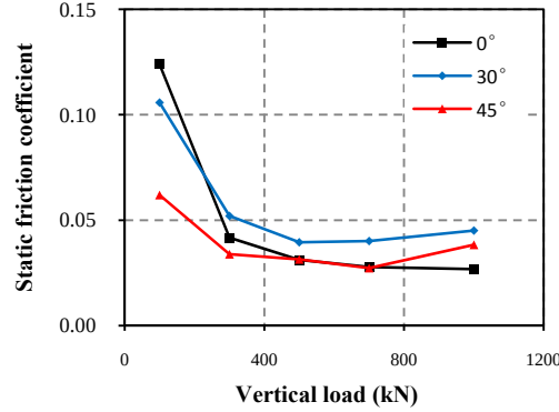
Figure 4: Static friction coefficient under different vertical load
