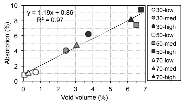
Figure 8: Relationship between calculated void volume and water absorption
