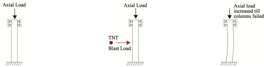
(a) Pre blast loading stage (b) Blast loading stage (c) Post blast loading stage
