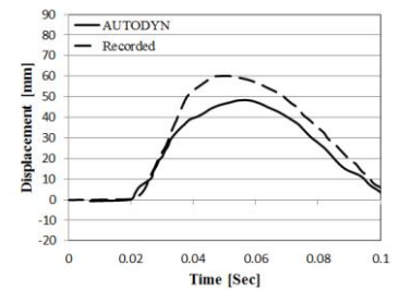
Figure 6: Deflection histories
