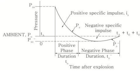
Figure 1: Free-field pressure-time variation (TM 5-855-1, 1986)
