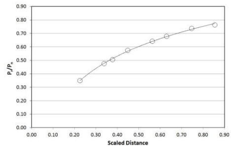
Figure 10: Relationship between reduction ratio of load capacity and scaled distance
