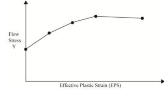
Figure 4: Yield stress versus effective plastic strain of Piecewise linear Johnson-cook model
