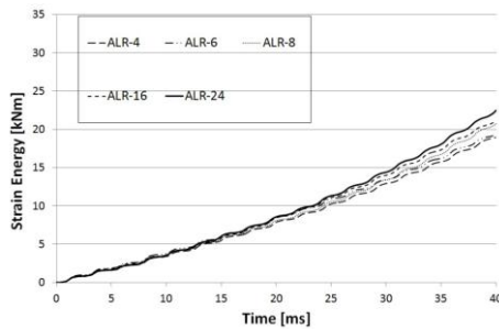
Figure 9: Effect of arrangement of longitudinal reinforcement on strain energy
