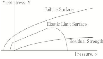
Figure 2: The RHT model used for concrete (Riedel et al., 2000)
