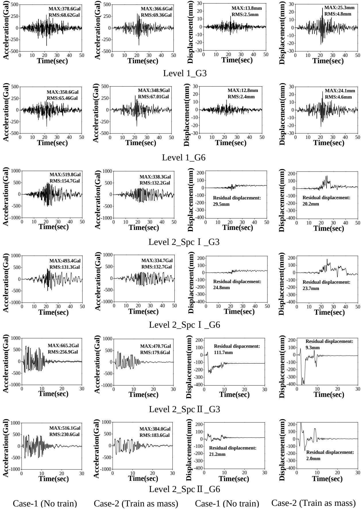
Figure 6: Seismic responses of bridge (horizontal acceleration and displacement).
