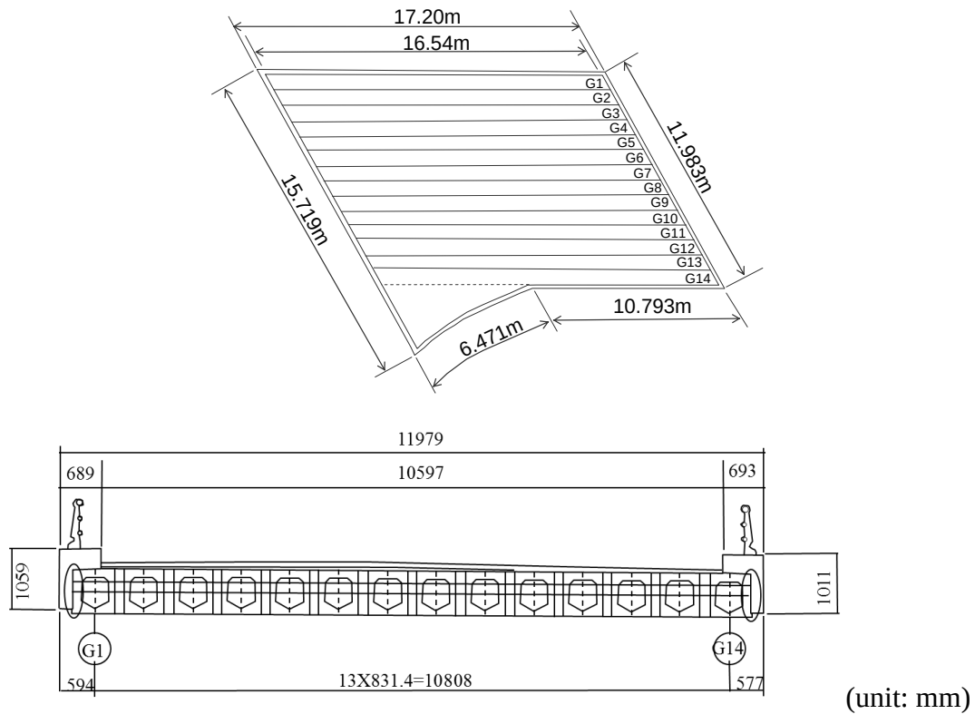
Figure 1. Top view and cross-section of bridge Y
