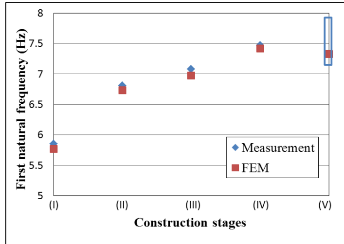
Figure 3. Comparison between measurement and FEM results of five construction stages
