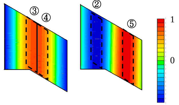
Figure 5. Contour plot of mode shape
