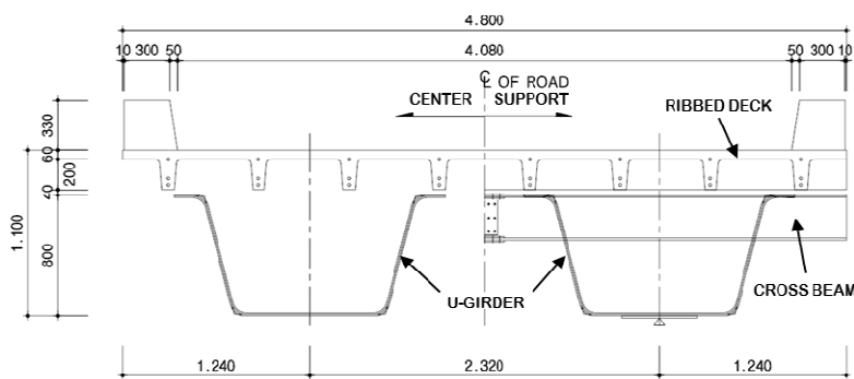
Figure 3: Composition of the trial bridge.
