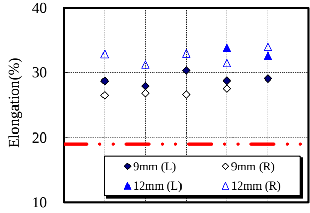
Figure 5: Elongation
