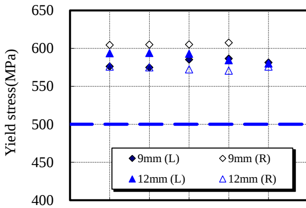
Figure 2: Yield stress
