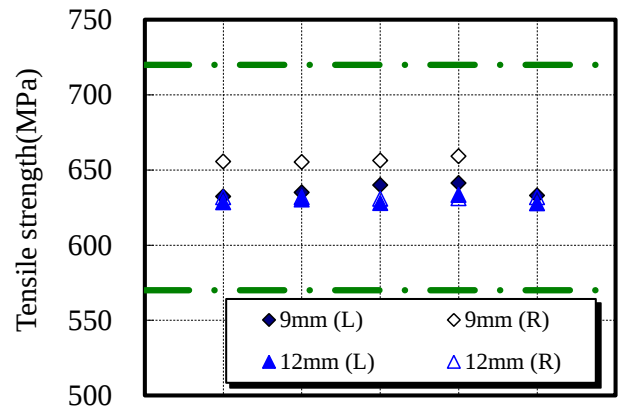
Figure 3: Tensile strength
