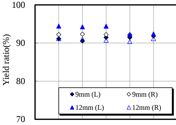
Figure 4: Yield ratio
