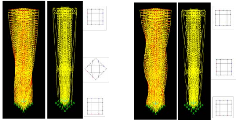
Figure 4: 60-story outrigger structures of two different rates of twist.
