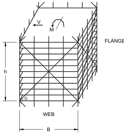
Figure 2: Typical braced tube module.
