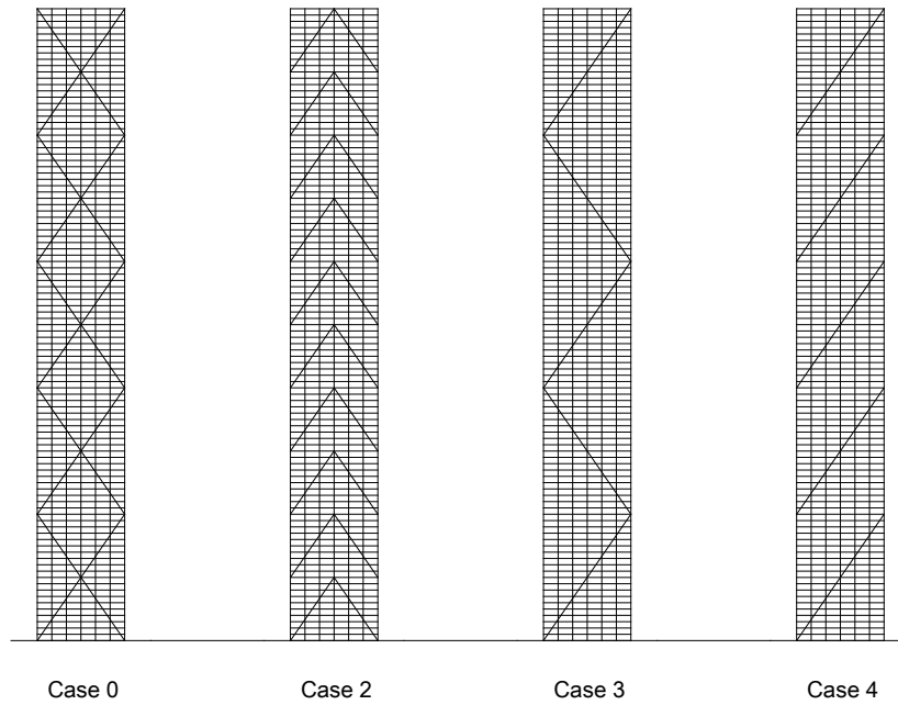
Figure 3: Braced tubes with chevron and single diagonal bracings.
