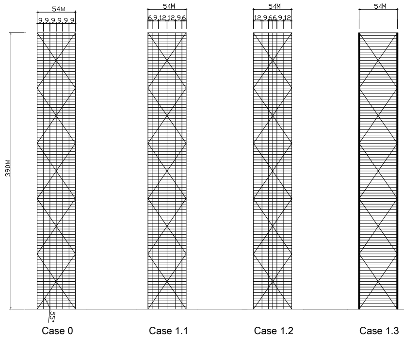
Figure 1: 100-story braced tubes of various column spacings.
