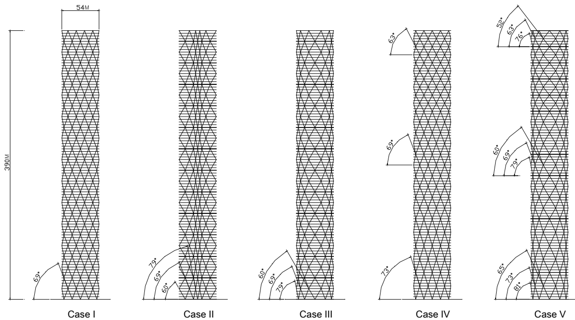
Figure 5: Diagrids of various angle configurations.
