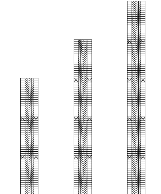
Figure 6: Outrigger Structures of 60, 80 and 100 Stories.
