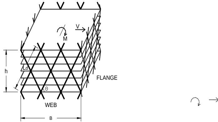
Figure 4: Typical diagrid module.
