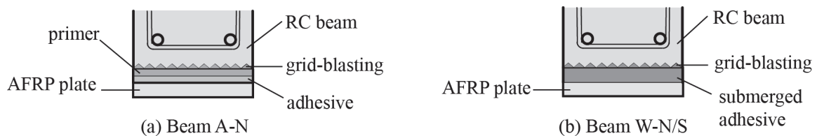
Figure 1: Schematic diagram of cross section
