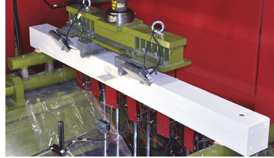
Photo 2: Experimental setup
