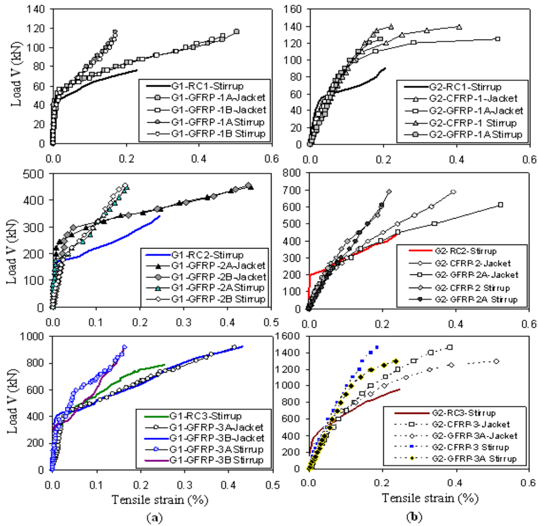
Fig. 5: Load –strain diagrams of FRP jacket and stirrups: (a) group G1; (b) group G2
