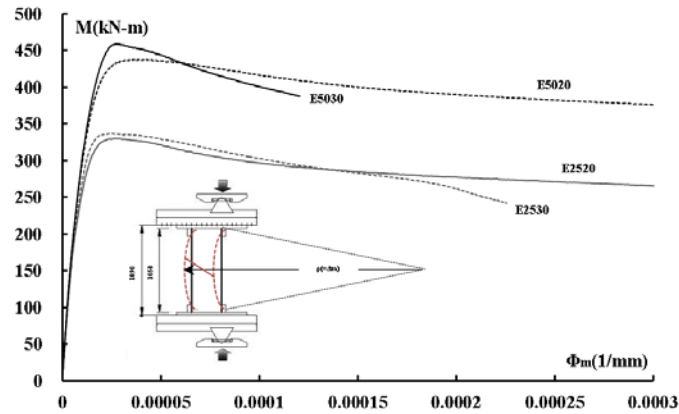
Figure 6: Moment-curvatures curve
