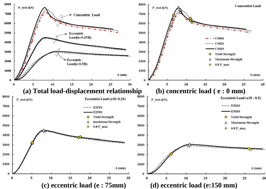
Figure 3: Load-displacement relationship
