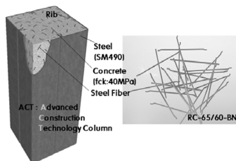
Figure 1: Concept of advanced construction technology column
