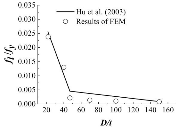
Figure 3: Comparison of confinement stress with results of Hu et al. (2003).
