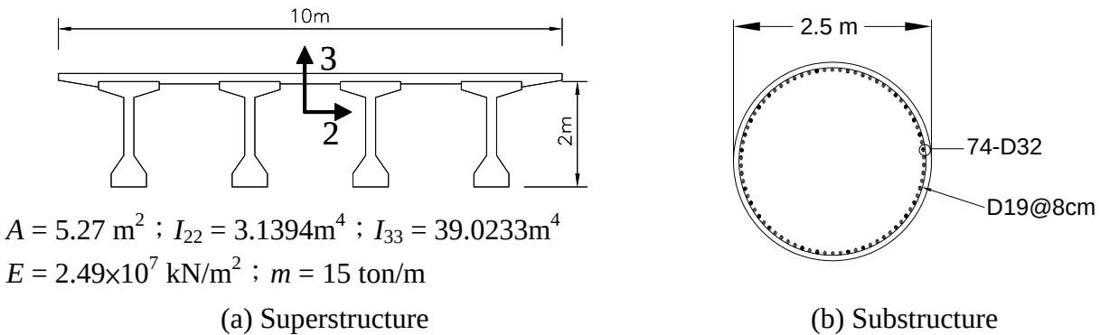
Figure 3: The cross section of the reference bridge.
