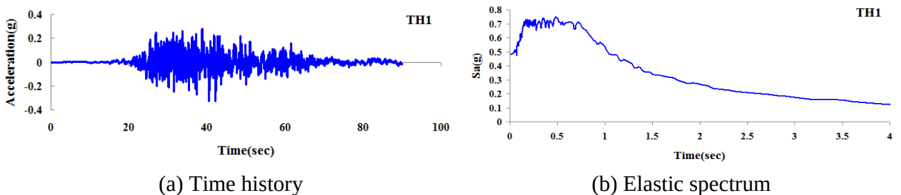
Figure 5: Typical time history and the corresponding elastic spectrum of DBE.
