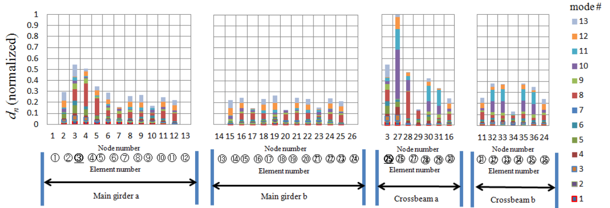
Figure 9: Damage index d_n and contribution ratio of each mode in C1
