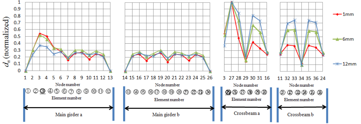
Figure 8: Damage index d_n in damage scenario C
