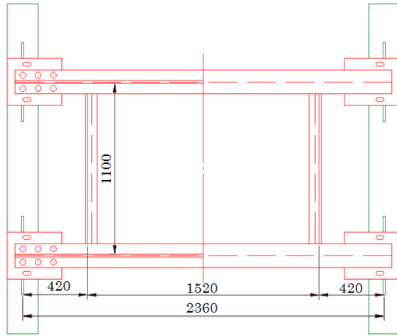
(a) Plan view (mm)
