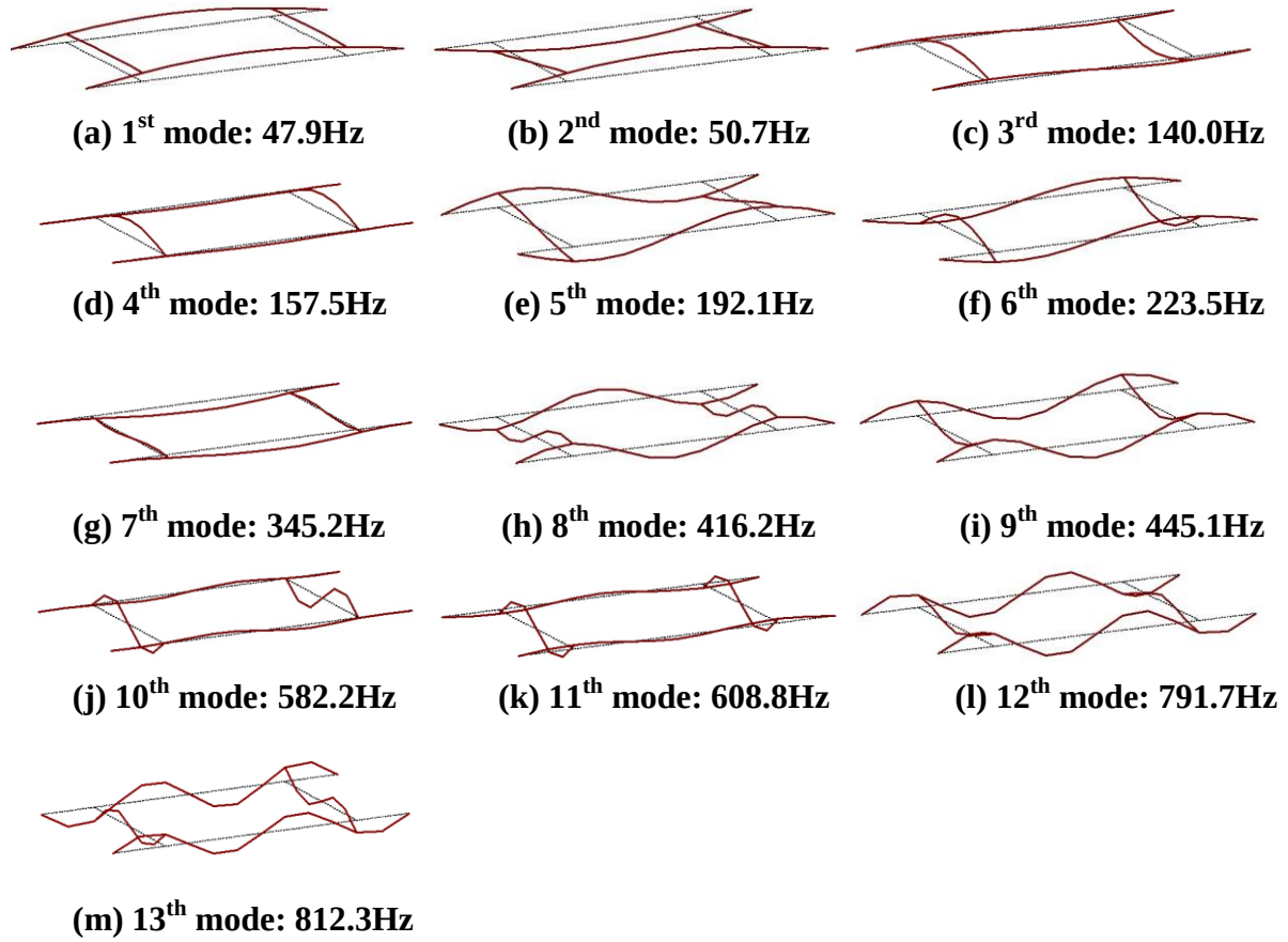
Figure 5: Natural frequencies and mode shapes
