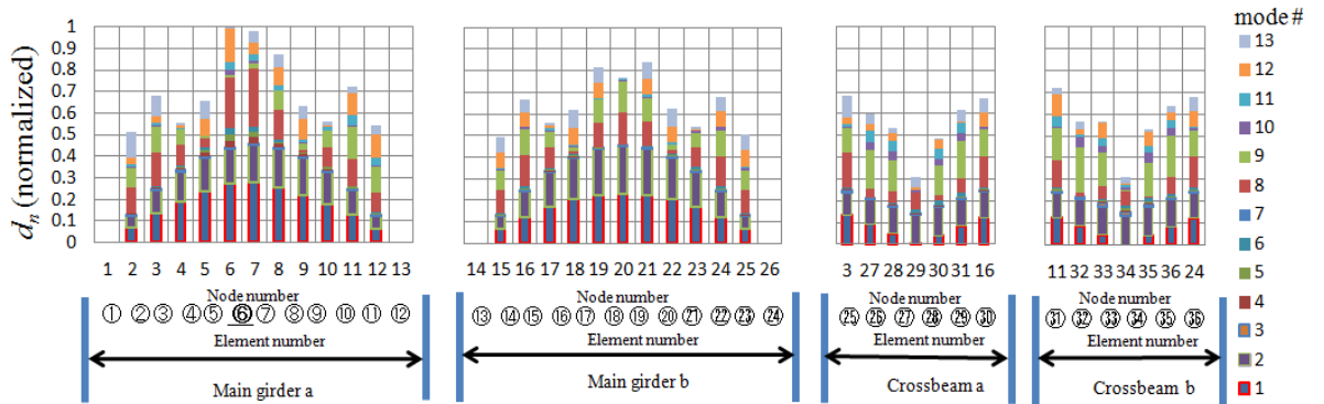
Figure 10: Damage index d_n and contribution ratio of each mode in A1
