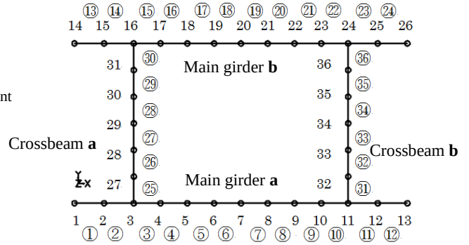
Figure 4: Node numbers and element numbers (Circled)
