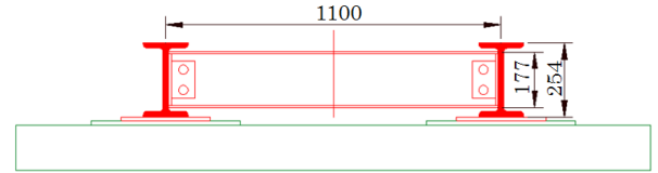
(c) Cross section (mm)
