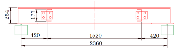
(b) Side view (mm)
