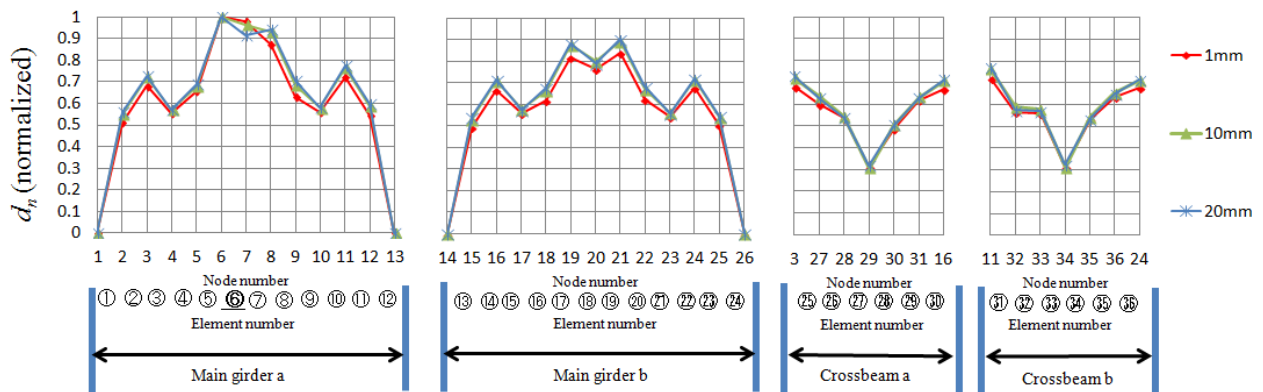
Figure 6: Damage index d_n in damage scenario A
