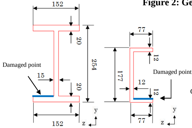
(a) Main girder
