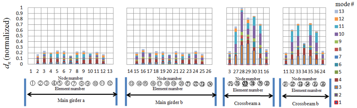
Figure 11: Damage index d_n and contribution ratio of each mode in B1
