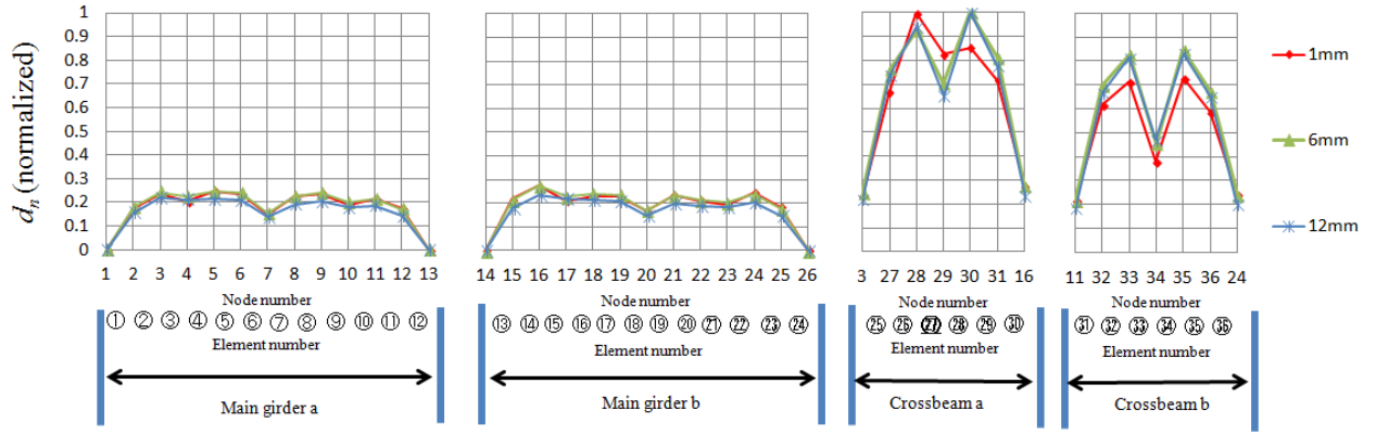
Figure 7: Damage index d_n in damage scenario B
