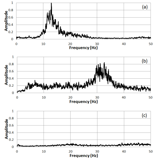
Fig. 4: Ground vibration test: (a) inflatable, (b) rubber, (c) PU.
