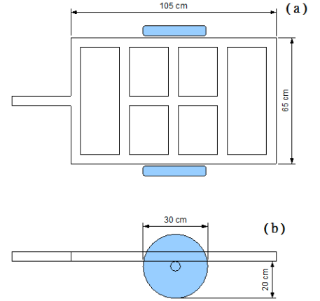
Fig. 1: Hand-drawn cart.
