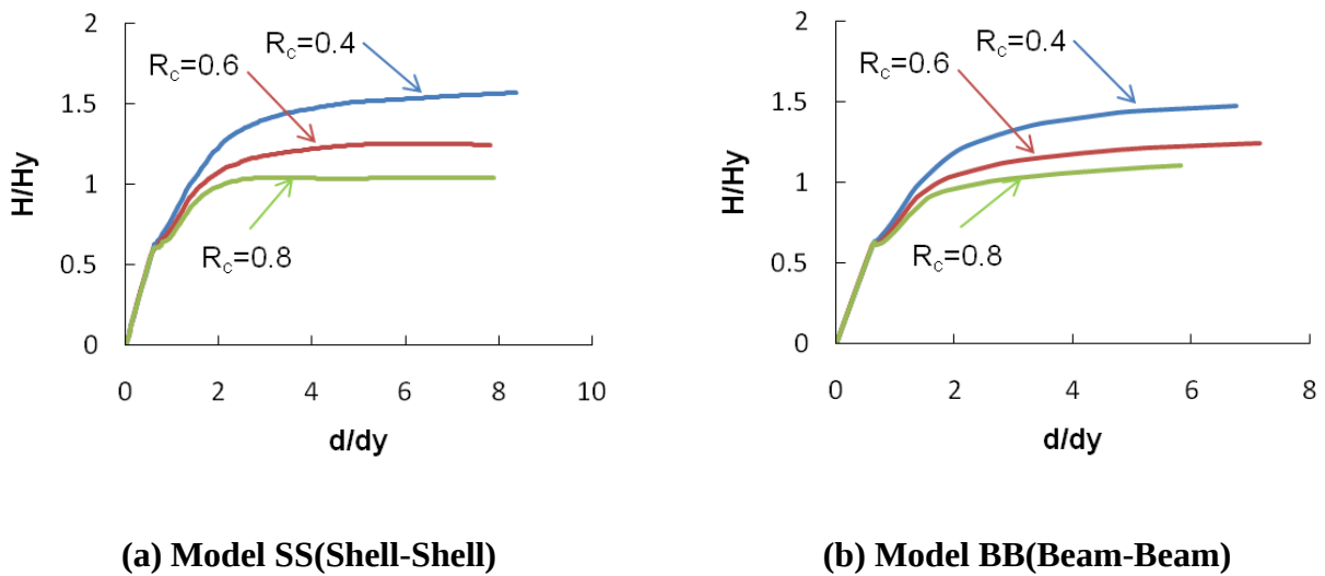
Figure 6: Lateral behavior of structure; brace specification: R_f=R_w=0.4 , L/r=100
