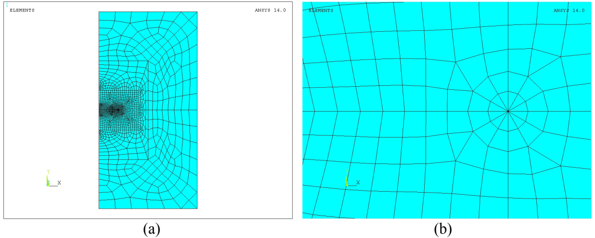
Figure 4: Finite element model. (a)half model, (b)local mesh.
