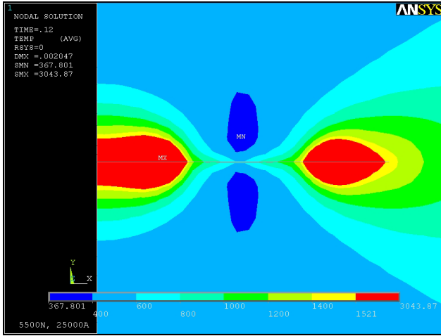
Figure 8: Crack welding.
