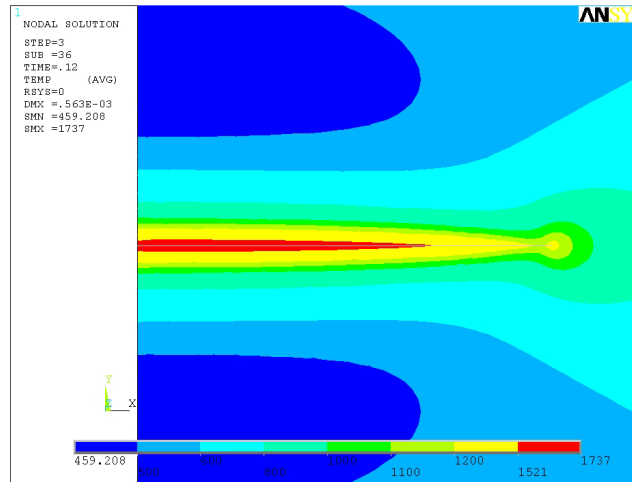
Figure 10: Result from constant \eta_{cel} .
