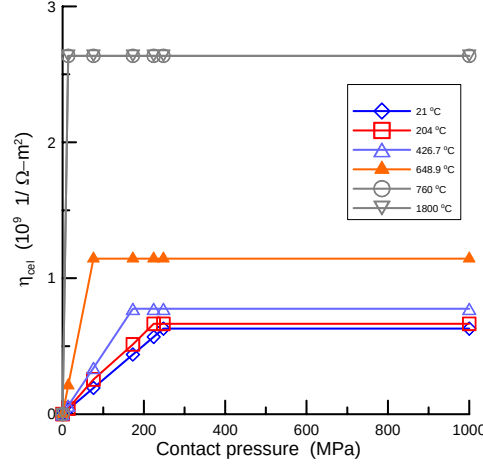
Figure 3: Pressure-dependent and temperature-dependent electrical contact conditions.
