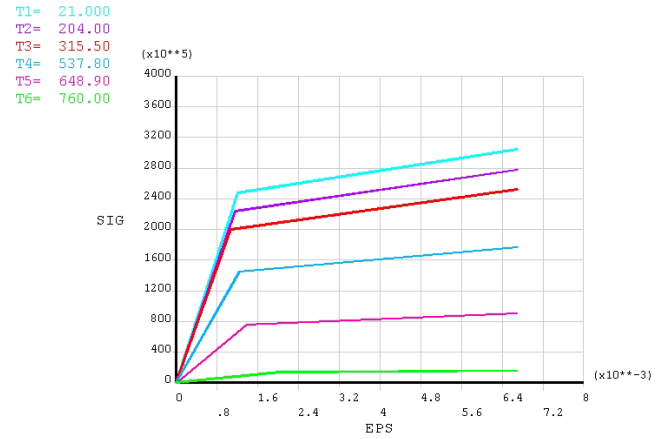
Figure 2: Elasto-plastic stress-strain.
