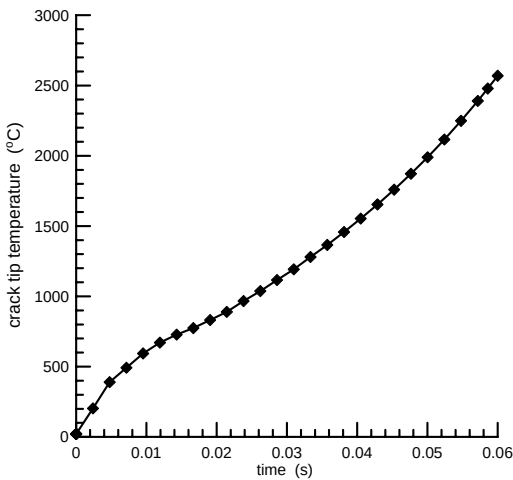
Figure 5: Crack tip temperature.
