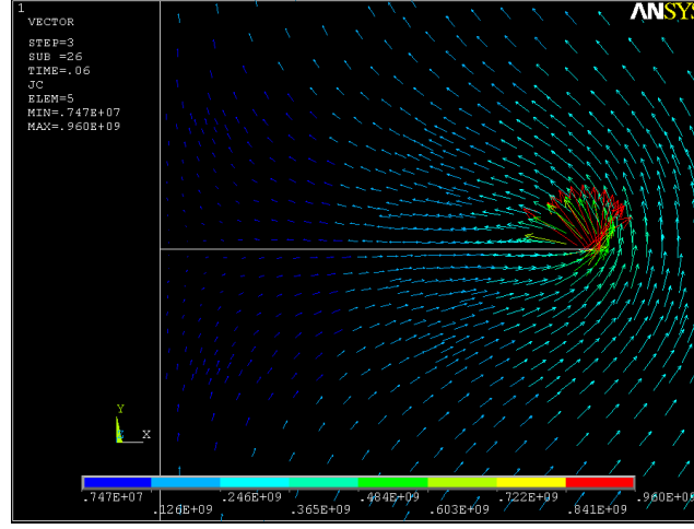
Figure 7: Electric current density vectors.
