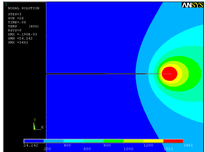
Figure 6: Temperature contour.
