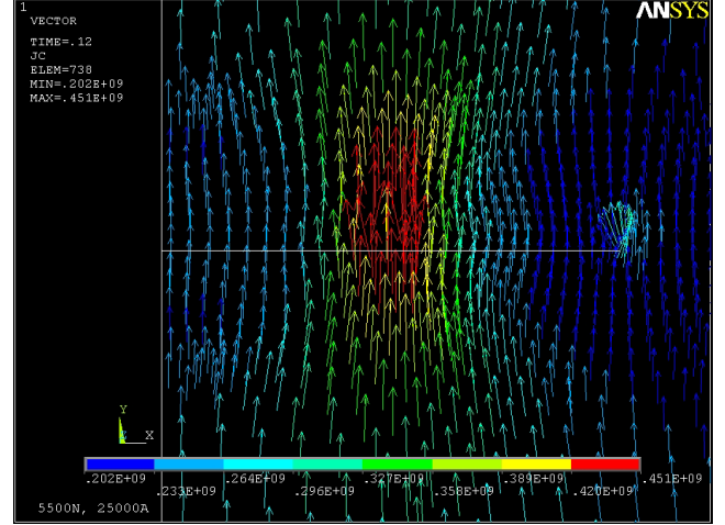
Figure 9: Electrical contact.
