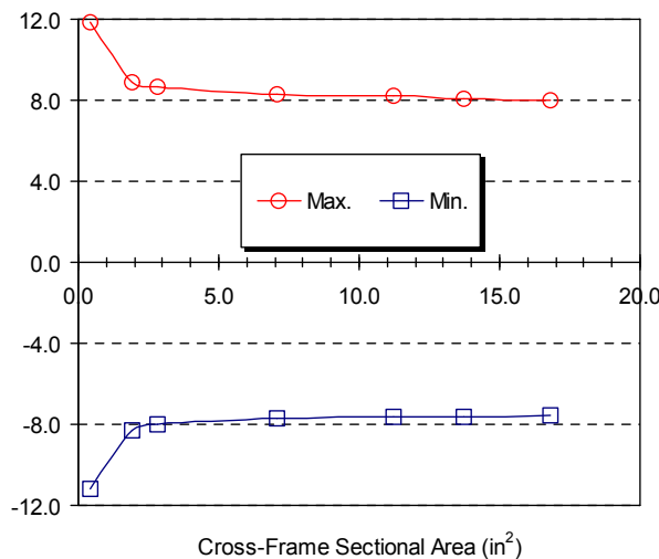
(a) along with Cross-Frame Sectional Area
