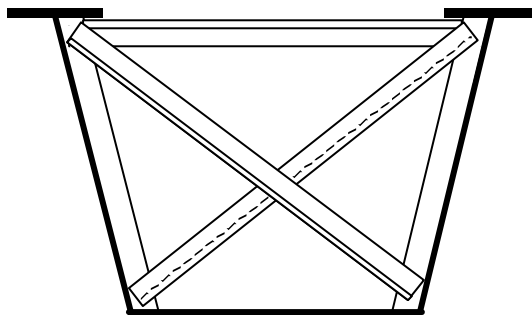
Figure 1: Cross-sections of Curved Box Girder Model
