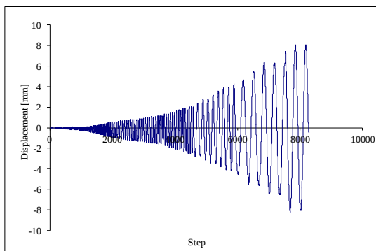
Figure 14. Load history
