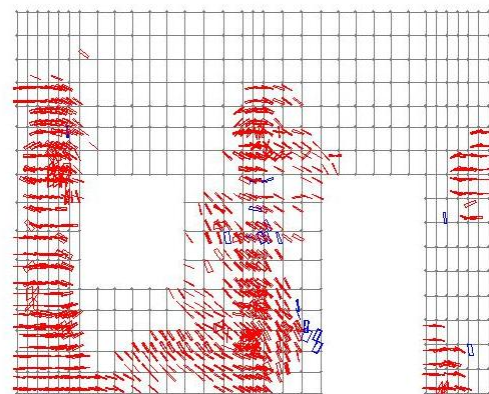
Figure 11. Numerical cracking pattern
