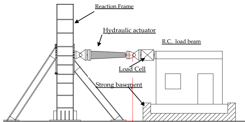
Figure 1. Overview of the test apparatus
