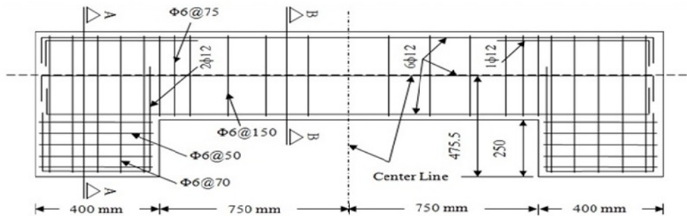
Figure 1: Geometry and reinforcements detail of columns (units in millimeters)
