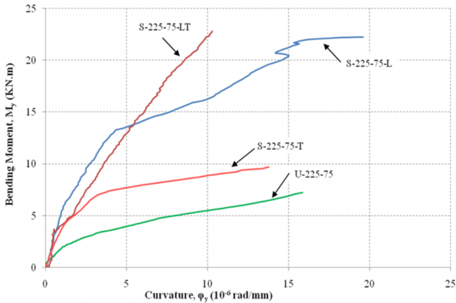
Figure 4: Moment-curvature behavior of the columns around the weak axis
