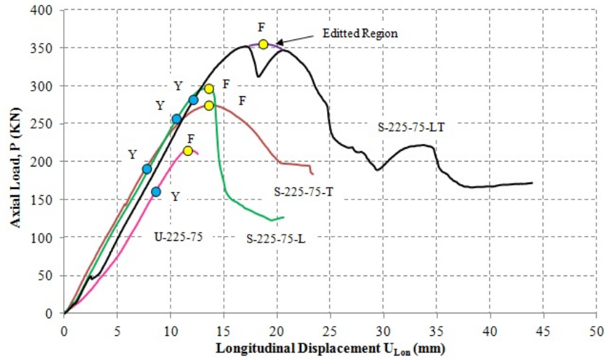
Figure 3: Load-displacement curves of the specimens
