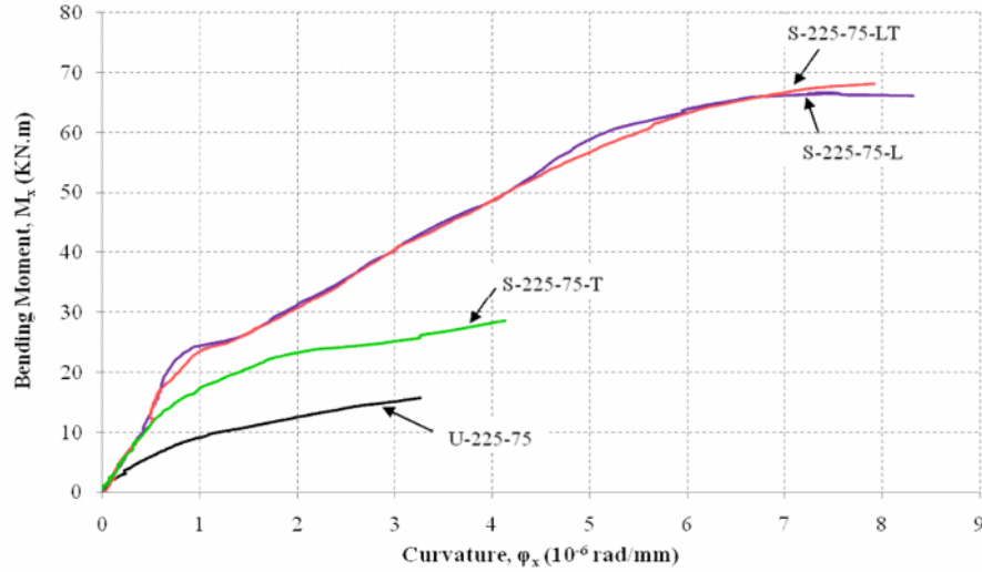
Figure 5: Moment-curvature behavior of the columns around the main axis
