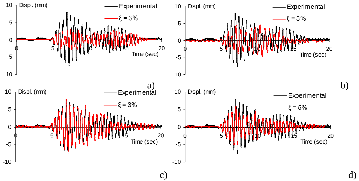
Figure 5. Comparison between dynamic test and numerical results for 00196 (intensity 25%).
