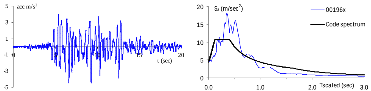
Figure 4: Accelerogram 00196x and comparison with considered elastic Code Spectrum
