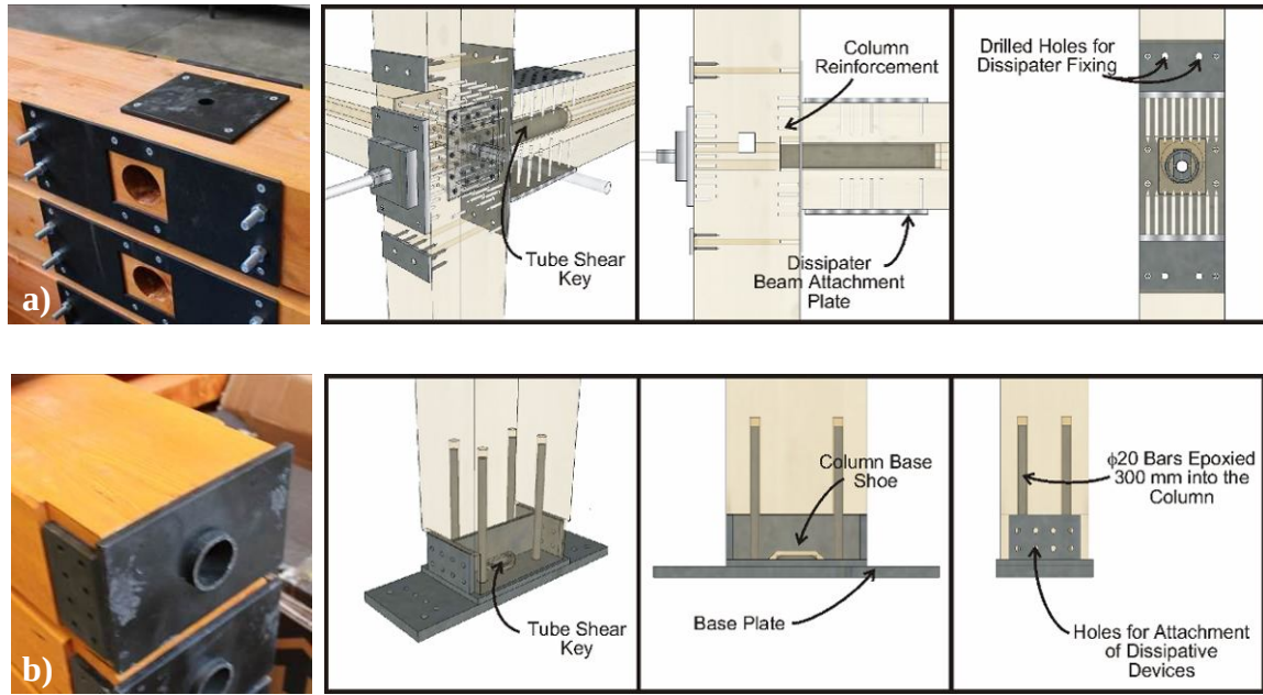
Figure 3: Post-tensioned Connections a) Beam to column and b) Column-Foundation.
