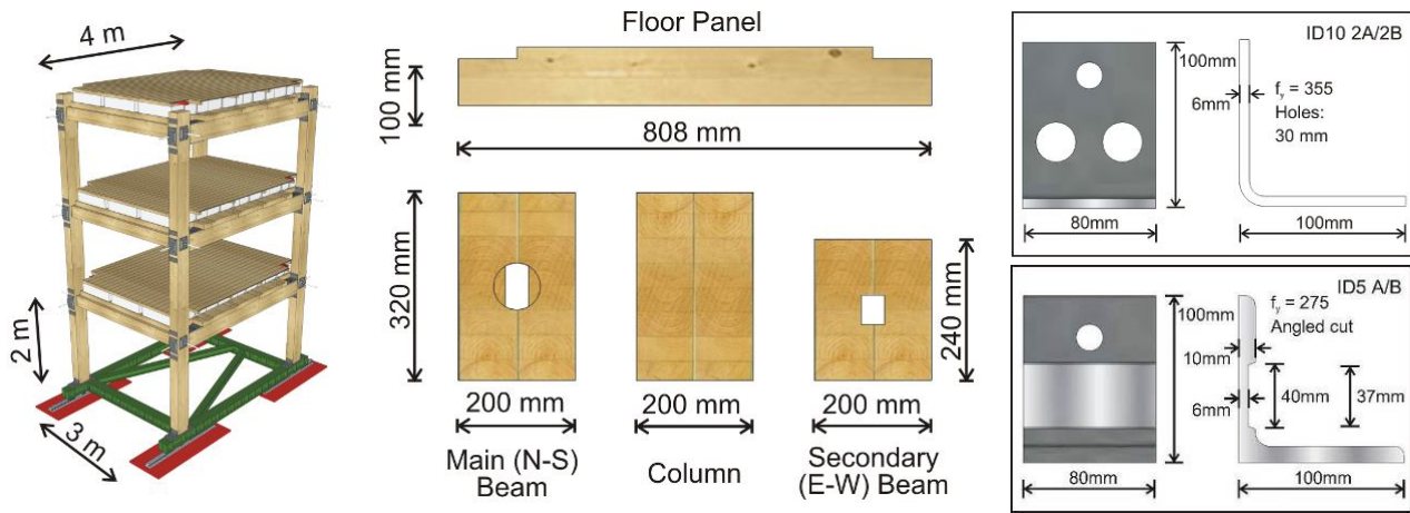
Figure 2: Test model overview and detailing and steel angle devices.
