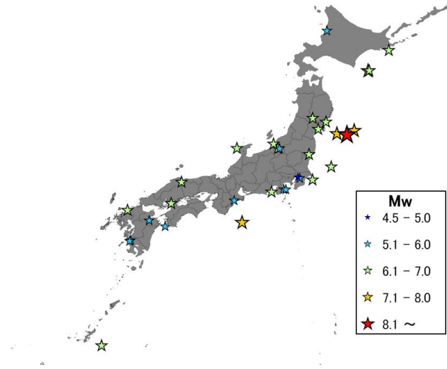
Figure 1: Locations of epicenters for the 32 earthquake events
