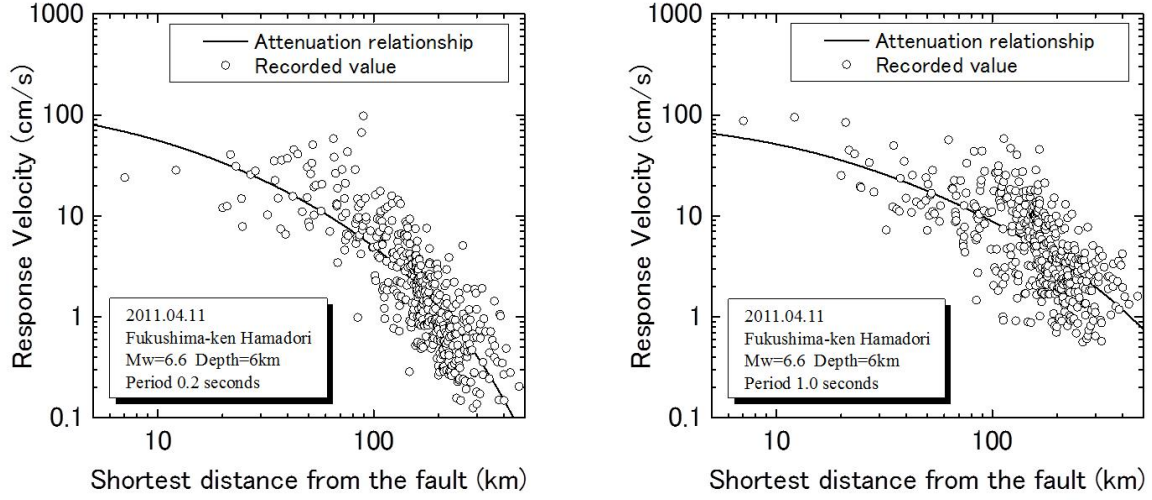
Figure 2: Attenuation relationship constructed by this study for a period of 0.2 s and 1.0 s
