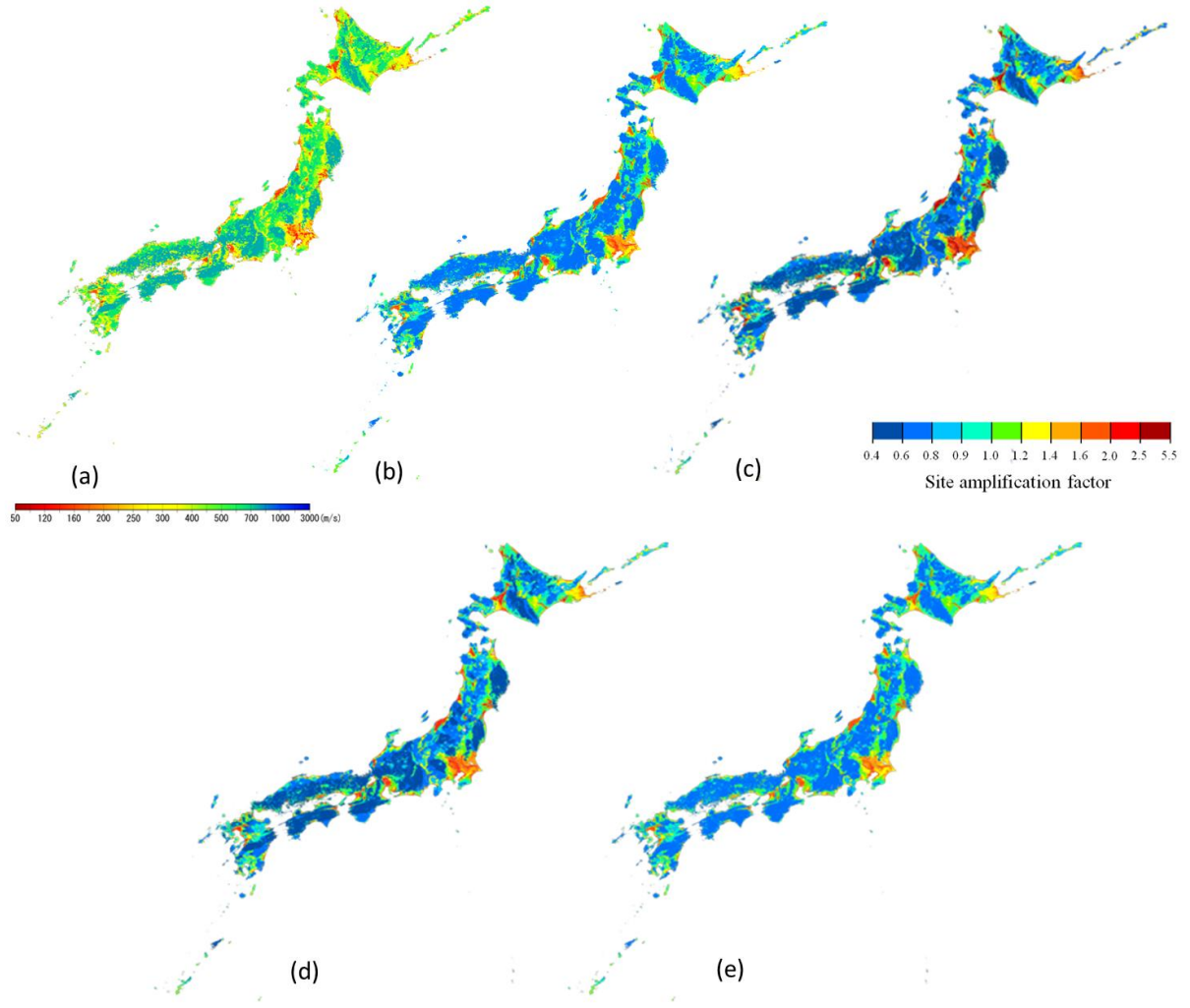
Figure 5: (a) Nationwide distribution of the AVS30 and those of the amplification factors of response spectrum for a period of (b) 0.5 s, (c) 1.0 s, (d) 2.0 s and (e) 5.0 s.
