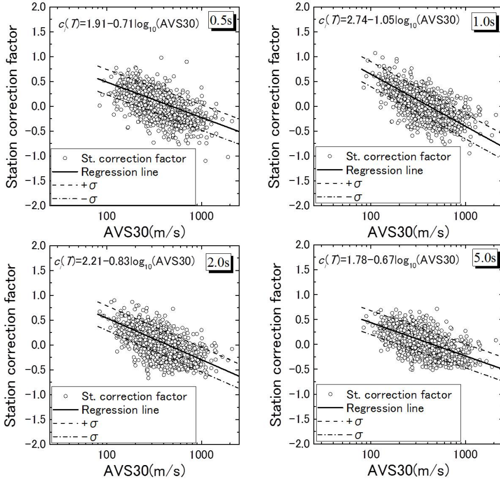
Figure 4: Relationship between the station correction factor and the AVS30 for a period of 0.5 s, 1.0 s, 2.0 s and 5.0 s
