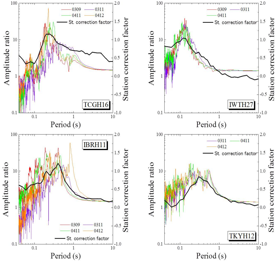
Figure 3: Comparison between the transfer functions for several dates (colored lines) and the station correction factor (black line) at KiK-net stations
