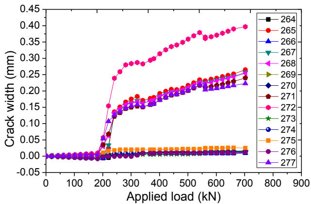
Figure 7 Load-crack width relationship in CB-1
