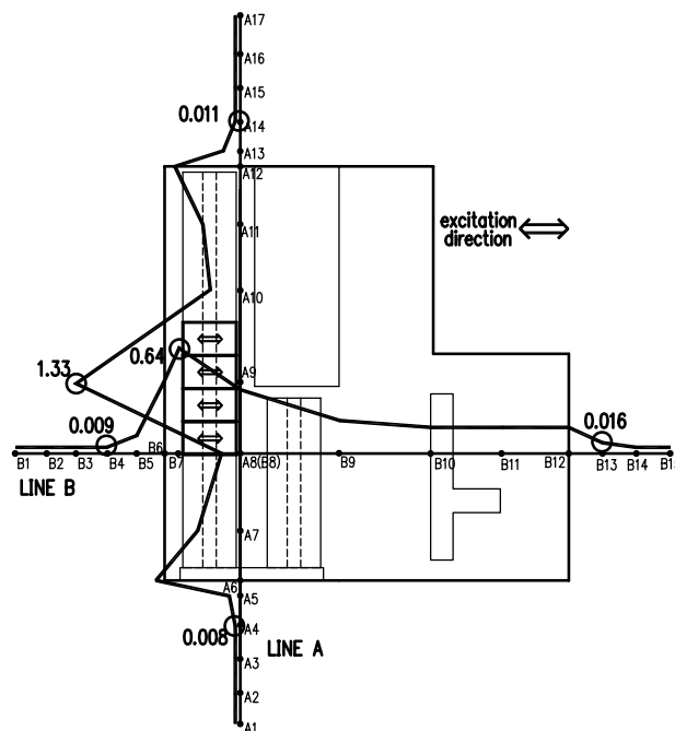
Figure 9: Peak transverse acceleration along line A and B for condition WCN-2 (unit:m/s 2 )
