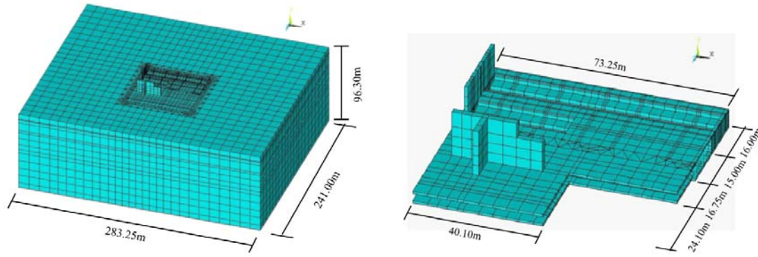
Figure 6: Finite element model and details of the concrete part
