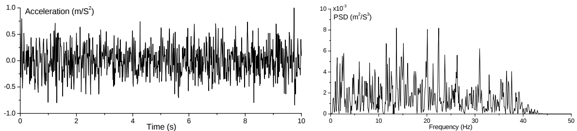
Figure 4: Time history and power spectral density of the excitation on table 2
