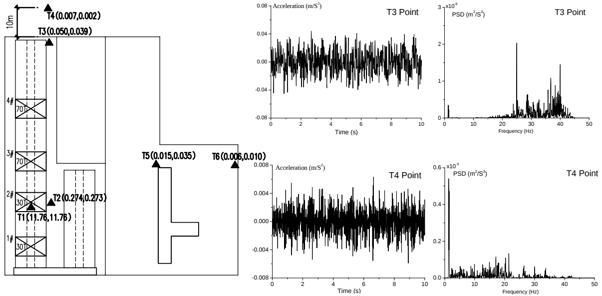
Figure 5: Peak acceleration and transverse acceleration of T3 and T4 (unit:m/s 2 )
