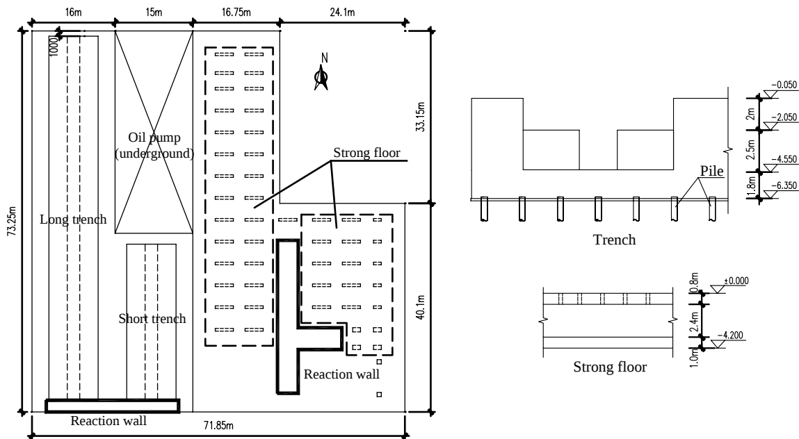
Figure 2: Layout of the large mass foundation and section of the trench and strong floor
