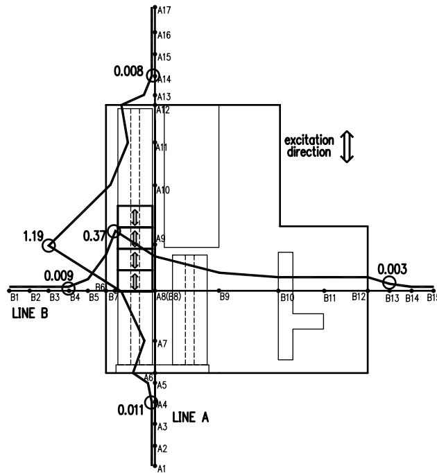
Figure 8: Peak longitudinal acceleration along line A and B for condition WCN-2(unit:m/s 2 )
