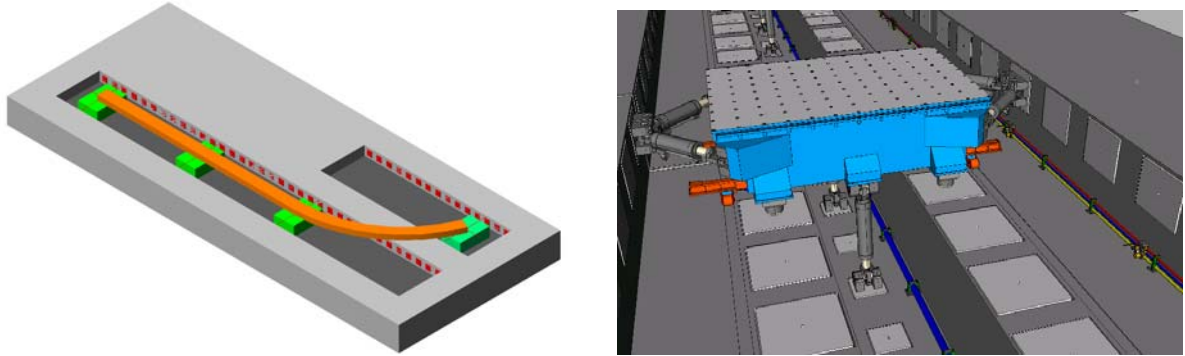
Figure 1: 4 movable shaking tables and 2 trenches
