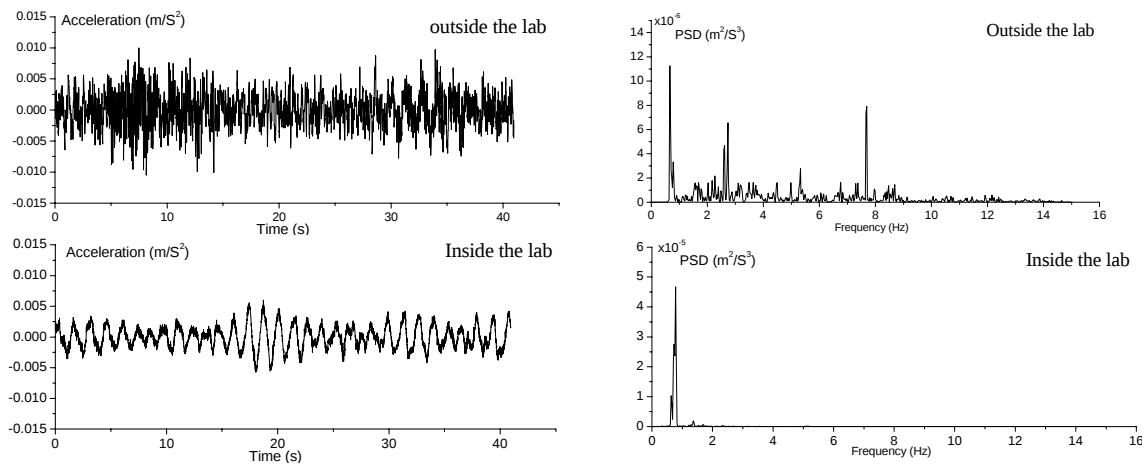
Figure 3: Time history and power spectral density of ground borne horizontal vibration
