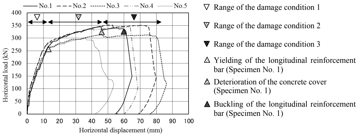
Figure 2: Load-displacement curves
