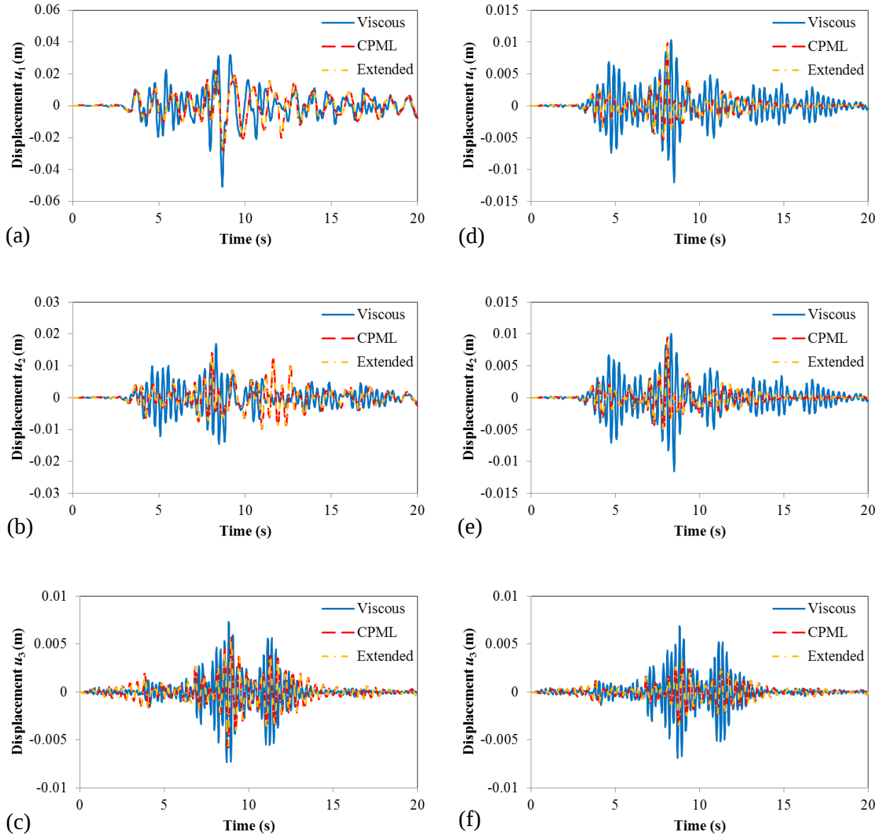
Figure 5: Responses of the roof of the building (left) and the center of the footing (right)
