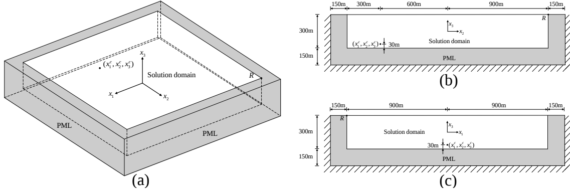
Figure 1: C-PML model for a three dimensional domain subjected to a point source.
