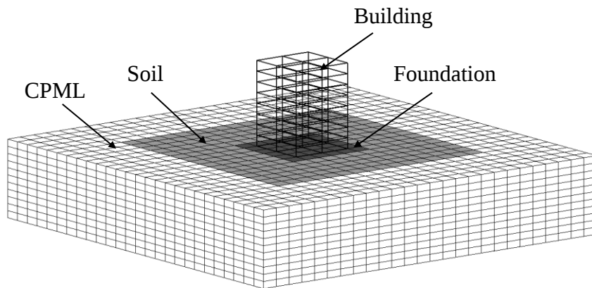
Figure 4: Finite element model of the soil-foundation-structure system with CPML
